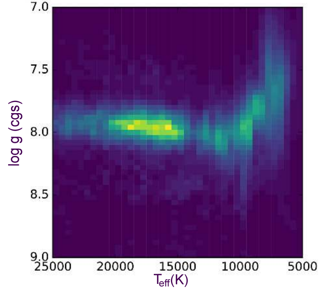
Figure 6. Hess diagram — density distribution — across effective temperature and surface gravity for DAs with spectra with S/N \geq 10 , showing the low mass DA white dwarfs concentrate below T_{\text{eff}} = 10000 K.
