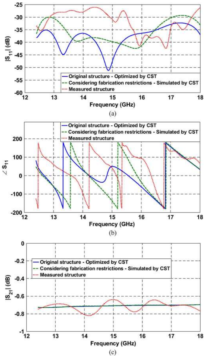
Fig. 9. Comparison between the S-parameters of the original transition optimized in CST (solid lines), the structure considering manufacturing restrictions, simulated in CST (dashed lines), and the measurement data (dotted lines): (a) reflection coefficient (amplitude); (b) reflection coefficient (phase); (c) transmission coefficient (amplitude).
