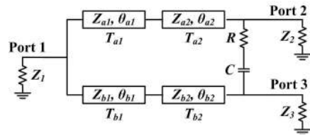
Figure 2. Constant VSWR-type three-port 3-dB power divider (CVT3PD) [31].
