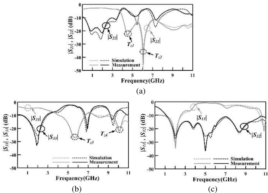
Figure 19. The measured and simulated scattering parameters of the proposed unequal-split power divider in Figure 18. (a) |S_{21}| and |S_{22}| . (b) |S_{31}| and |S_{33}| . (c) |S_{11}| and |S_{32}| .
