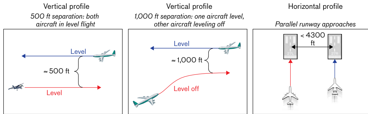
FIGURE 10. Shown here are the three main encounter types representing the majority of U.S. TCAS alerts.
