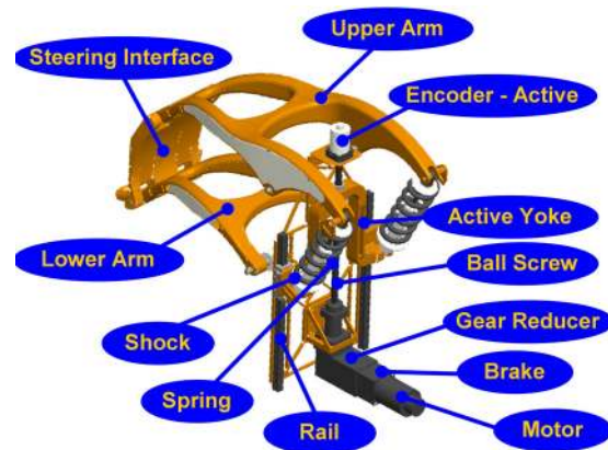
Figure 6. Suspension system.
