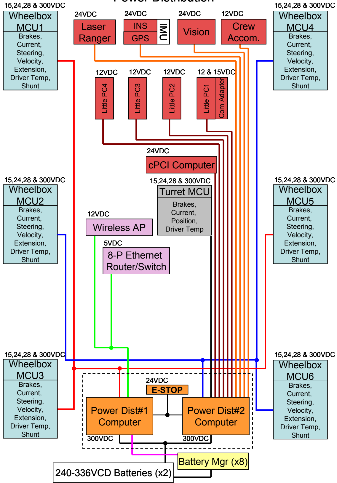
Figure 12. Power distribution unit.
