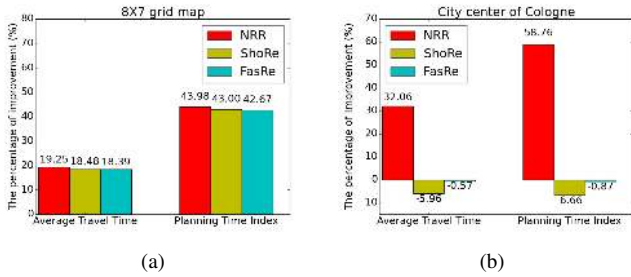
Fig. 9: Comparison of the percentage of improvement achieved by NRR, ShoRe and FasRe over ERE in terms of ATT and PTI
