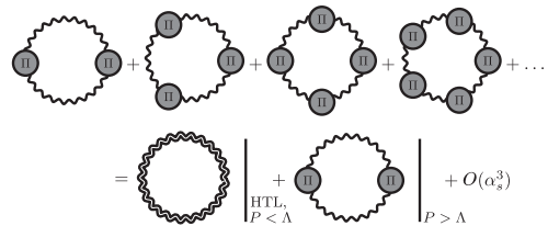
FIG. 1. Graphical representation of Eq. (3) after kinematic simplifications are employed. See the text for an explanation.
