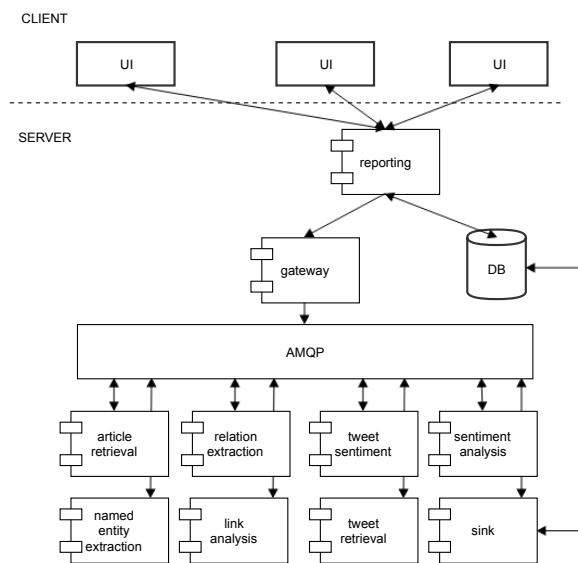
Figure 1: Architecture of the novel AML framework.
