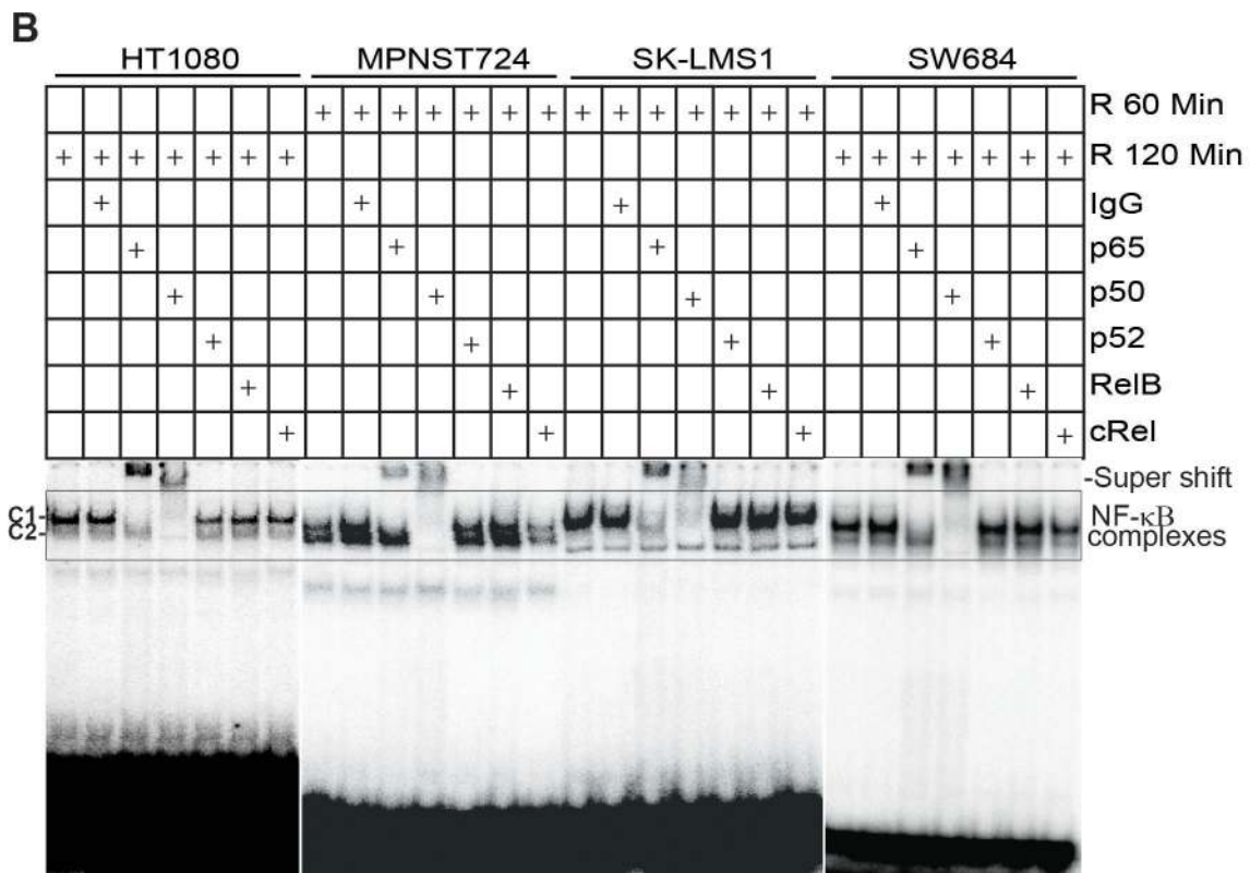
Figure 6: Radiation activates the canonical NF-κB. A. Tumor cells were irradiated at a dose of 50 Gy and nuclear extracts were prepared at 1 and 2 h after culture. Nuclear extracts were then analyzed for canonical NF-κB activity using EMSA with NF-κB consensus sequence-containing DNA probe as in Figure 3. Anti-p65 and anti-p50 antibodies were used to identify the canonical NF-κB-DNA complexes. C1: p65/p50 heterodimer complex; C2: p50/p50 homodimer complex. B. The tumor cells were irradiated and cultured for 1 and 2h, respectively. Nuclear extracts were then analyzed for NF-κB activation using EMSA as in A. Antibodies that are specific for the five indicated NF-κB Rel subunits (p65, p50, p52, RelB, and cRel) were used to identify the NF-κB-DNA complexes.
