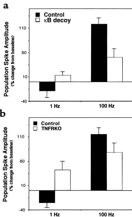
Figure 2 NF- \kappa B in synaptic plasticity. (a) Population spike amplitudes recorded from hippocampal slices from adult mice, pretreated with either scrambled control DNA or \kappa B decoy DNA and stimulated at either 1 or 100 Hz. Note that \kappa B decoy DNA prevents LTD of synaptic transmission induced by stimulation at 1 Hz and attenuated long-term enhancement of synaptic transmission induced by stimulation at 100 Hz. (b) Population spike responses recorded from hippocampal slices from wild-type mice (Control) and mice lacking TNF- \alpha receptors (TNFRKO) after stimulation at either 1 or 100 Hz. Note that LTD of synaptic transmission is not induced by stimulation at 1 Hz in slices from TNFRKO mice, and that long-term enhancement of synaptic transmission is attenuated in slices from TNFRKO mice. Modified from ref. 23.
