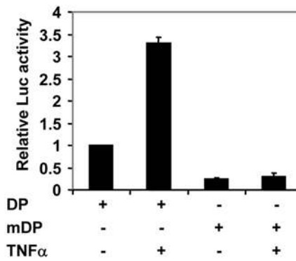
Figure 2. Effect of mutation of putative NF-κB site in optineurin promoter on TNF \alpha -induced activity. (A) Nucleotide sequence of human optineurin promoter. Putative transcription factor binding sites for various transcription factors such as Sp1, NF-κB, MyoD, HSF1, HSF2, NRSF and CREB are shown. The 5' mRNA (exon 1) sequence is shown in italics. First nucleotide of optineurin mRNA is taken as transcription start site (+1), indicated by an arrow. (B) Schematic representation of various promoter reporter constructs used for experiments in C, D. Full length promoter (FP), deleted promoter (DP) and their NF-κB site mutants mFP and mDP are shown. The nucleotide sequence of putative NF-κB site is shown and the 3 nucleotides which were mutated are underlined. (C) Mutant or normal full length optineurin promoter constructs (mFP or FP) were transfected in A549 cells and after 6 hours of transfection TNF \alpha was added. Cell lysates were prepared after 24 hours of transfection for reporter assays. Luciferase activities relative to untreated control promoter (taken as 1.0) are shown (n=3). (D), The same experiment as in (C) was carried out using deleted promoter, DP, or its mutant, mDP.
