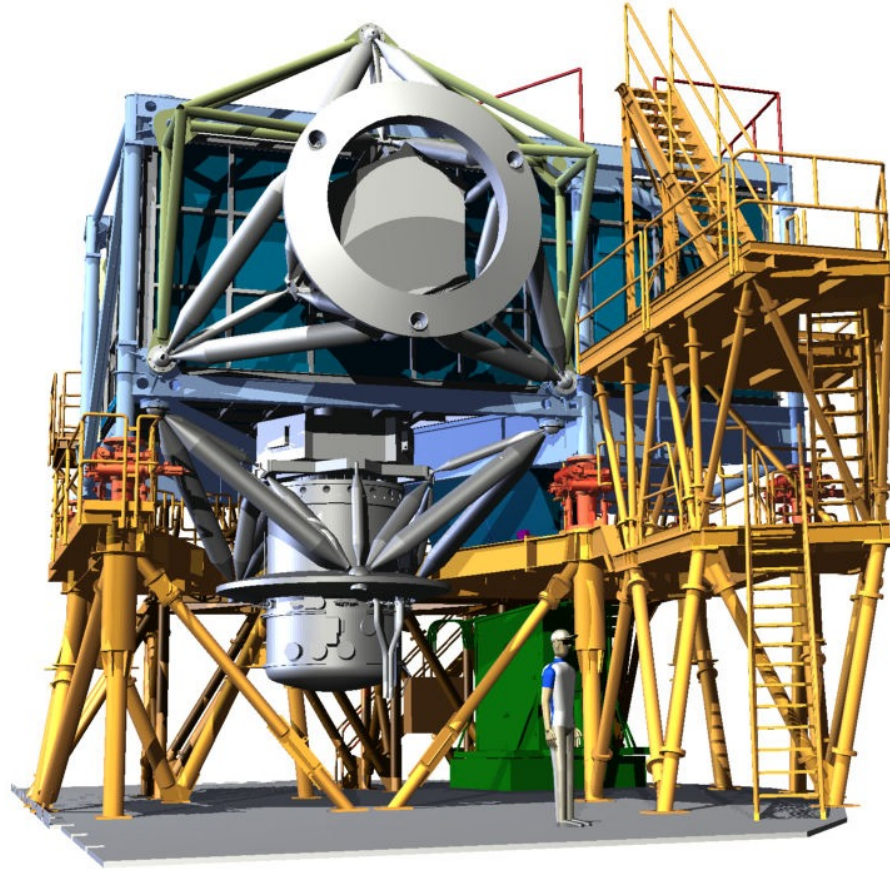
Figure 12: NFIRAOS on Nasmyth platform with IRIS underneath and NSEN on top
