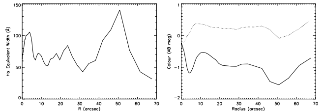
Figure 2. The H\alpha EW (radial) profile of NGC 922 is shown on the left-hand panel and radial colour profiles of NGC 922 are shown on the right-hand panel where the FUV–NUV and FUV – R colour profiles are represented by the dotted and solid lines, respectively.
