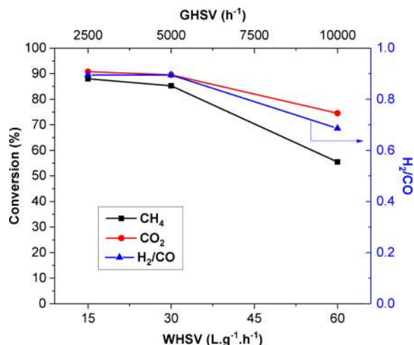
Fig. 6. Effect of the space velocity on H 2 /CO ratio and CH 4 and CO 2 conversion for LNz10. Reaction conditions: P = 1 atm, CH 4 /CO 2 = 1, T = 700 °C.
