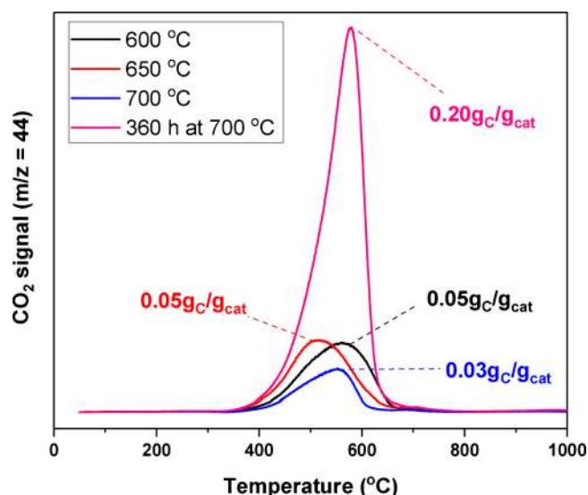
Fig. 9. TPO profiles of LN210 after DRM during 30 h at different temperatures and after 360 h at 700 °C.
