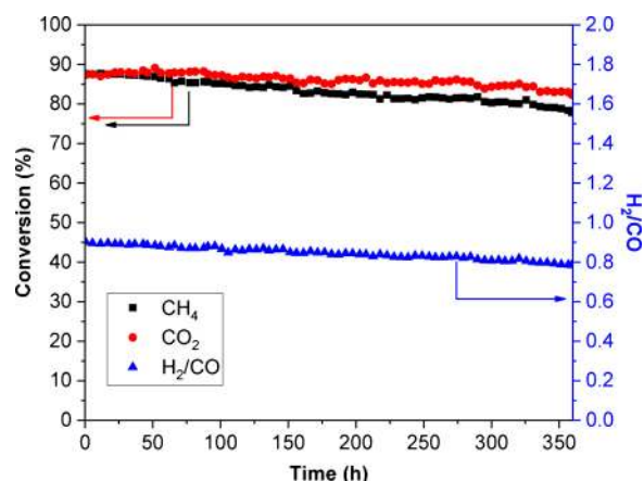
Fig. 7. Stability test on LNz10 over 360 h. Reaction conditions: CH 4 /CO 2 :1, P = 1 atm, T = 700 °C and WHSV = 30 L.g -1 .h -1 .
