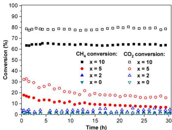
Fig. 4. Influence of Ni metal loading ( x = 0; 2; 5; 10 wt.% Ni) on catalytic activity and stability. Reaction conditions: P = 1 atm, \text{CH}_4/\text{CO}_2 = 1 , T = 650 °C, \text{WHSV} = 30 \text{ L.g}^{-1}.\text{h}^{-1} .
