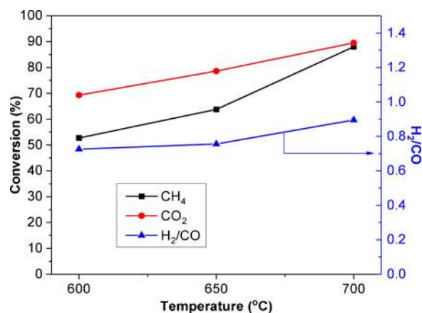
Fig. 5. Effect of the temperature on H 2 /CO ratio and CH 4 and CO 2 conversion for LNZ10. Reaction conditions: P = 1 atm, \text{CH}_4/\text{CO}_2 = 1 , \text{WHSV} = 30 \text{ L.g}^{-1}.\text{h}^{-1} .
