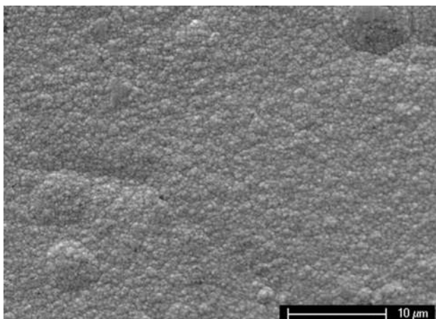
Fig. 1 SEM image of Ni-W (47.7 wt.% W) coating surface electrodeposited at a current density of 5 \text{ A/dm}^2
