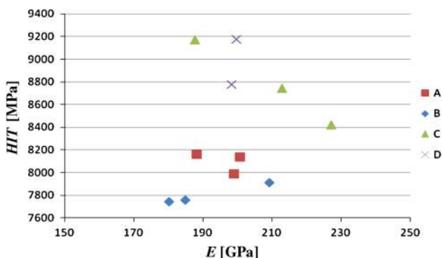
Fig. 7 Indentation hardness and Young's modulus
