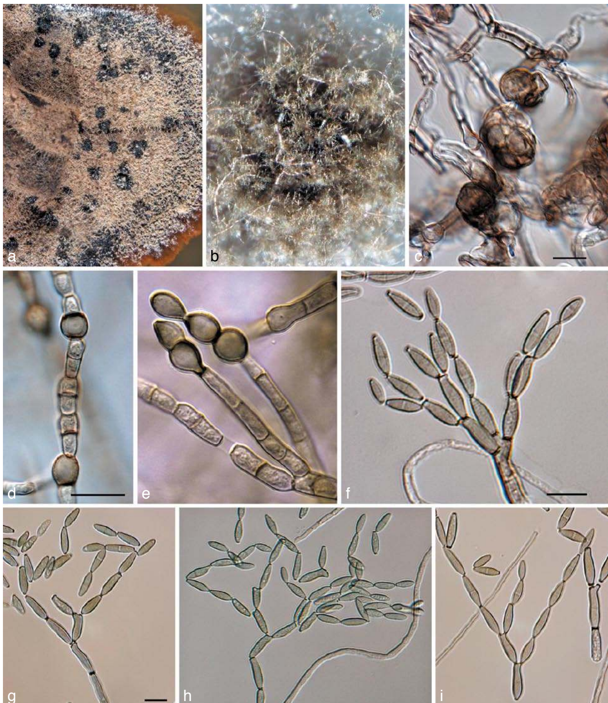
Fig. 7 Toxicocladosporium chlamydosporum (CPC 15709). a. Colony forming black sclerotial structures on MEA; b. sporulation on OA; c–e. micro-sclerotia and chlamydo-spore-like cells formed in culture; f–i. conidiophores with penicillate heads of branched conidial chains. — Scale bars = 10 µm.
