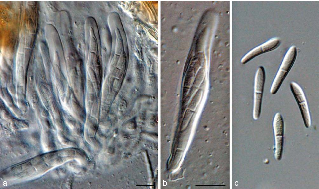
Fig. 3 Mycosphaerella marksii (CPC 14655). a. Asci in squashed ascoma; b. single ascus; c. ascospores with typical asymmetrical apical cells. — Scale bars = 10 μm.
