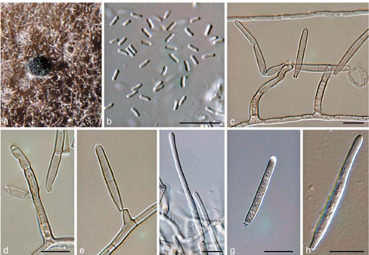
Fig. 4 Passalora intermedia (CPC 15745). a. Spermatogonium forming on OA; b. spermatia; c–f. conidiophores giving rise to conidia; g, h. conidia. — Scale bars = 10 μm.
