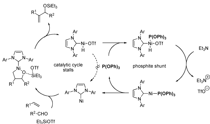
Scheme 9 Proposed mechanism for coupling of alkenes and aldehydes catalyzed by [\text{Ni}(\text{IPr})\{\text{P}(\text{OPh})_3\}] .
