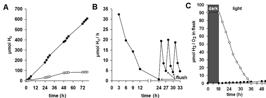
Figure 2. (A) H 2 evolution data for water (○) and 20% aqueous methanol (●) using 100 mg nanosheets. (B) Rate of H 2 evolution from Pt-[HfCa 2 Nb 3 O 10 ] as a function of time. Arrows indicate evacuation to 20 torr followed by purging with Ar gas. (C) Evolution of H 2 (●) and of added O 2 (○) under irradiation.
