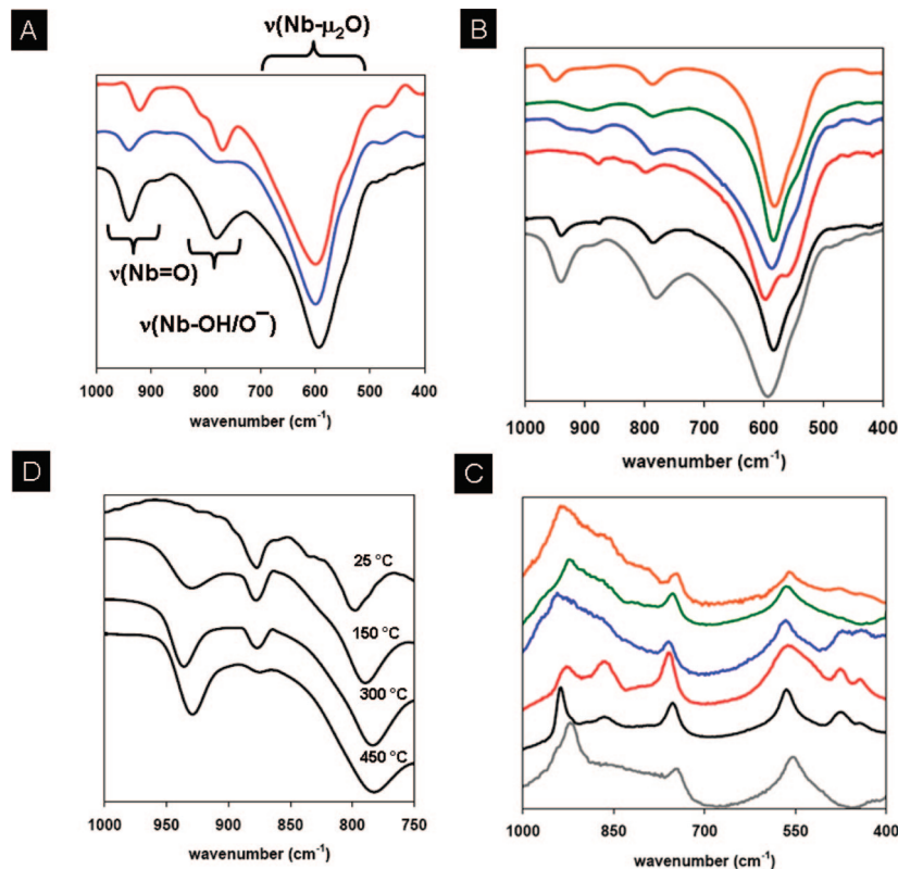
Figure 4. (A) Infrared spectra of \text{KCa}_2\text{Nb}_3\text{O}_{10} (top), \text{HCa}_2\text{Nb}_3\text{O}_{10} (middle), and \text{TBACa}_2\text{Nb}_3\text{O}_{10} (bottom). (B) IR and (C) Raman spectra of \text{TBACa}_2\text{Nb}_3\text{O}_{10} before (gray) and after (black) irradiation in \text{H}_2\text{O} , after storage (green) and irradiation (blue) in \text{H}_2^{18}\text{O} , after treatment with \text{H}_2\text{O}_2 (red), and after irradiation in air (orange). (D) IR showing thermal removal of \text{H}_2\text{O}_2 .
