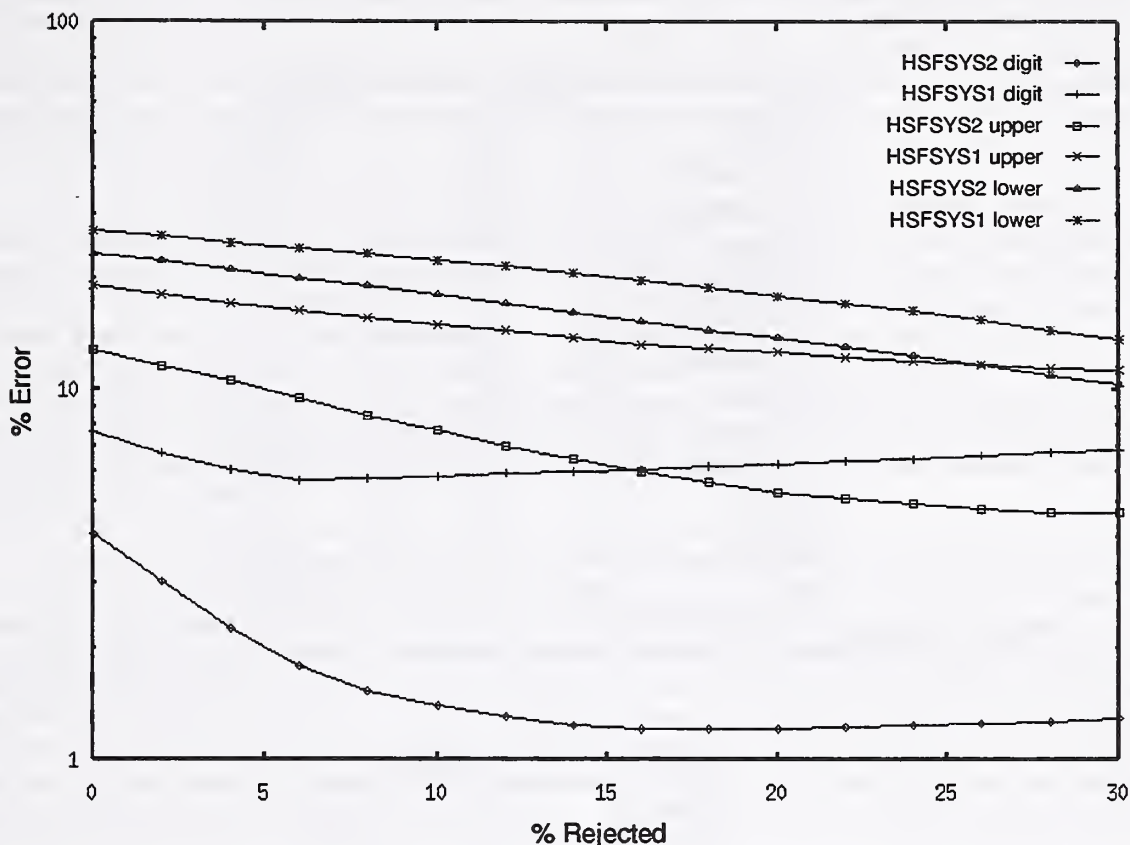
Figure 11. Error versus rejection rates for digit, upper, and lowercase recognition between HSFSYS1 and HSFSYS2.
