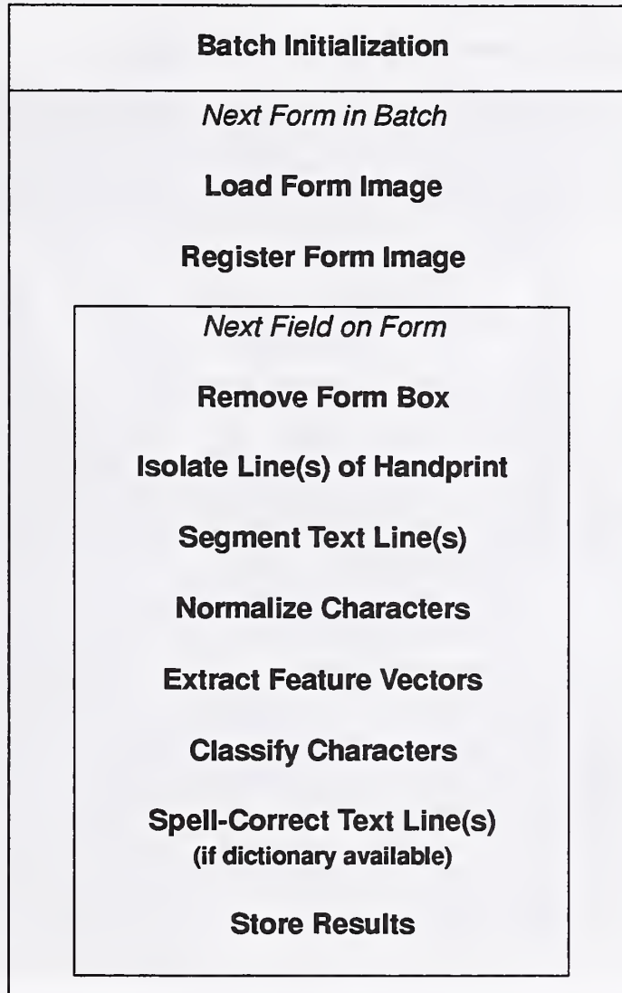
Figure 4. Organization of the functional components within the new recognition system.
