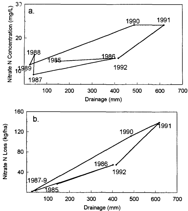
Fig. 3. Relationship between subsurface tile drainage and (a) annual flow-weighted nitrate N concentration and (b) annual nitrate N loss in file drainage water from continuous corn that received 200 kg N/ha each spring at Waseca, MN.
