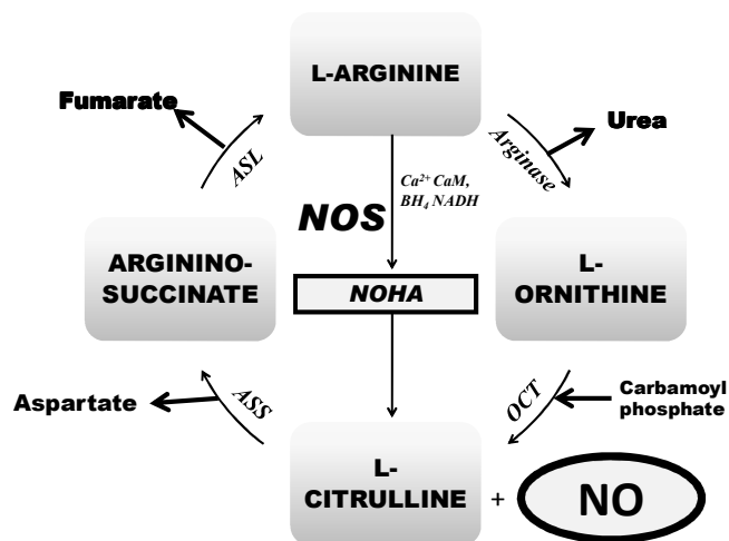
Figure 1 Production of nitric oxide. Nitric oxide synthases (NOS) catalyze an oxidation of one N^{\circ} -atom of the guanidine group of L-arginine to form NO (nitric oxide) and L-citrulline, with the intermediate N^{\circ} -hydroxy-L-arginine (NOHA). ASS, argininosuccinate synthase; ASL, argininosuccinate lyase; OTC, ornithine carbamoyltransferase.
