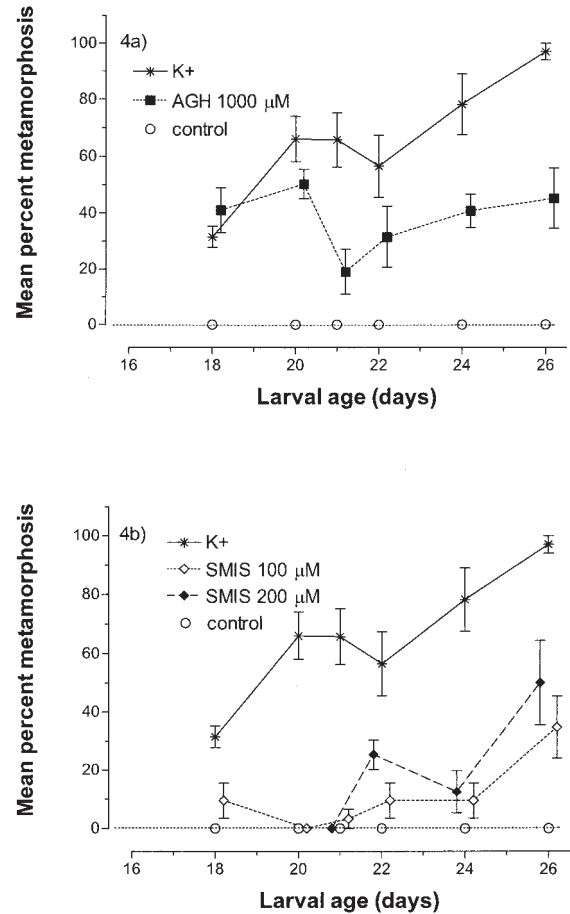
Figure 4. Development of responsiveness to excess \text{K}^+ and to the nitric oxide synthase inhibitors (a) AGH (aminoguanidine hemisulfate) at 1000 \text{ μmol l}^{-1} and (b) S -methylisothiourea sulfate (SMIS) at 100 and 200 \text{ μmol l}^{-1} in larval cultures of Crepidula fornicata . Data shown are the mean responses ( \pm 1 SD) after 24 h of exposure. See Table 1 for additional details (Experiment VI).
