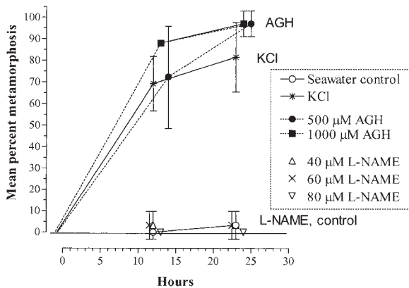
Figure 3. Effects of the nitric oxide synthase inhibitors aminoguanidine hemisulfate (AGH) and L - N^G -nitroarginine methyl ester ( L -NAME) on metamorphosis of Crepidula fornicata larvae. Each point represents the mean response ( \pm 1 SD) of four replicates of eight larvae each. Excess \text{K}^+ served as a positive control. No larvae metamorphosed when tested at an L -NAME concentration of 10 or 20 \text{ μmol l}^{-1} (data not shown). See Table 1 for data on larval age and shell length for these experiments (Experiment V).
