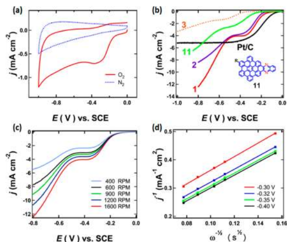
Figure 3. (a) CV curves (scanning rate of 50 \text{ mV s}^{-1} ) of 1 on a glassy-carbon RDE in a \text{N}_2 - and an \text{O}_2 -saturated 0.1 \text{ M KOH} solution. (b) LSV curves ( 10 \text{ mV s}^{-1} ) for 1–3 and Pt/C on a RDE (1600 rpm) in an \text{O}_2 -saturated 0.1 \text{ M KOH} solution. Also shown is the LSV curve for 11 , a much smaller N-substituted heterocycle with structure shown in the inset. (c) LSVs ( 10 \text{ mV s}^{-1} ) for 1 on a RDE in an \text{O}_2 -saturated 0.1 \text{ M KOH} solution with various rotating speeds. (d) Koutecky–Levich plots for 1 obtained from the LSV curves in (c) at various voltage values. A global fitting of the plots reveals that the number of electrons transferred per \text{O}_2 molecule is 3.9.
