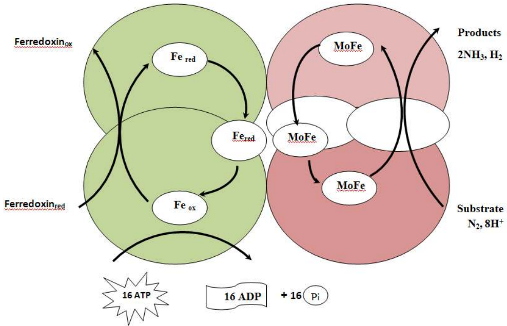
Figure 3. The structure of nitrogenase
