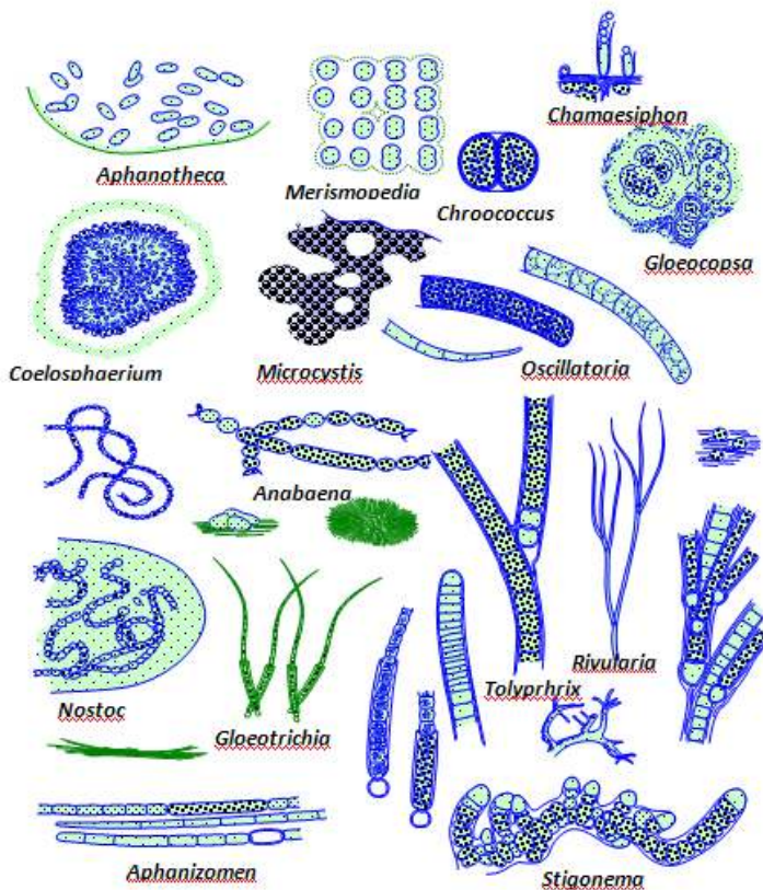
Figure 1. N 2 -fixing cyanobacteria
