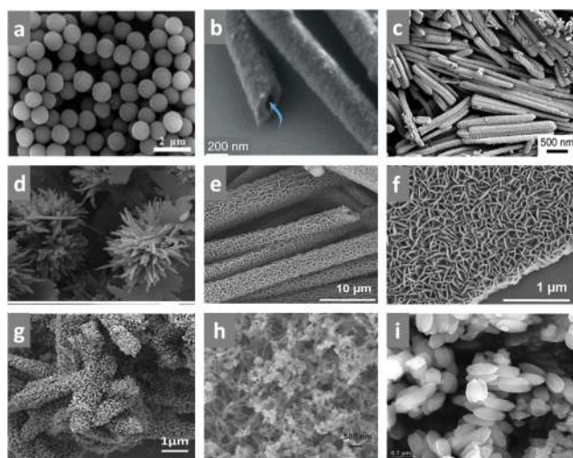
Fig. 32 FESEM images showing different surface morphologies of COFs. Reproduced with permission from: (a) ref. 186, Copyright the American Chemical Society (2019); (b) ref. 187, Copyright John Wiley and Sons (2018); (c) ref. 141, Copyright the American Chemical Society (2019); (d) ref. 68, Copyright the American Chemical Society (2019); (e and f) ref. 188, Copyright Elsevier (2019). (g) ref. 138, Copyright The Royal Society of Chemistry (2021); (h) ref. 189, Copyright the American Chemical Society (2017) and (i) ref. 57, Copyright The American Association for the Advancement of Science (2020).
