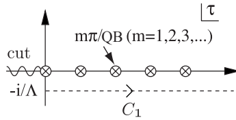
Fig. 1. The contour of the integration in Eq. (2.5). The circles denote the poles.
