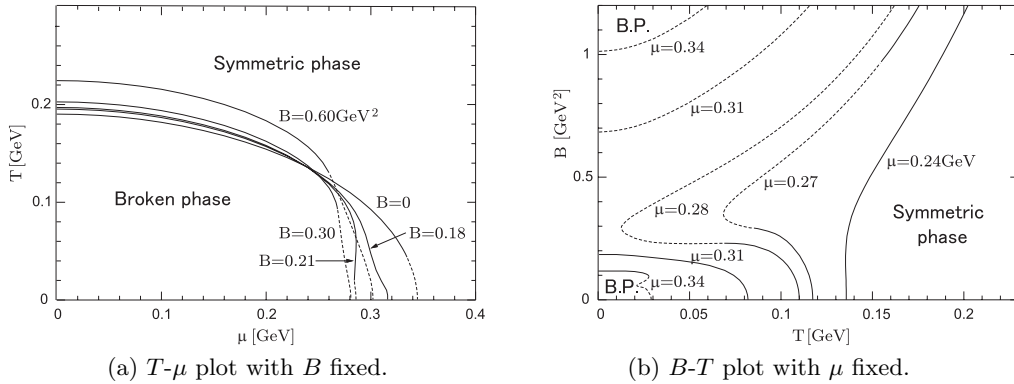
Fig. 2. Critical lines on T - \mu plane and B - T plane. The dashed line represents the first order phase transition while the solid line represents the second order phase transition.
