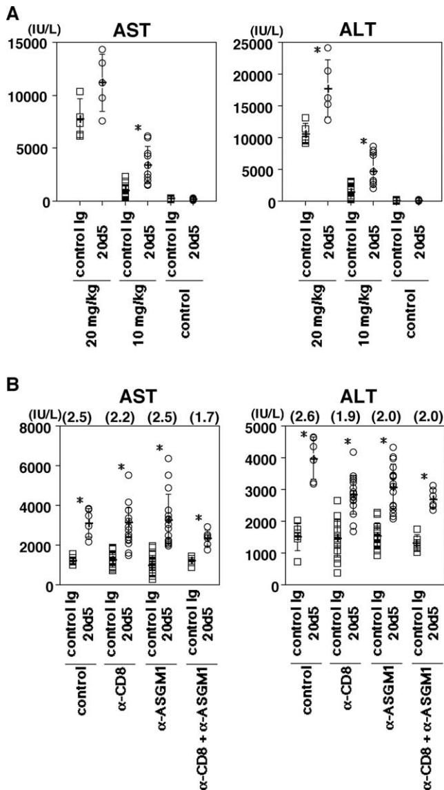
FIGURE 2. Augmented serum AST and ALT levels following Con A injection by NKG2A signal blockade. A , Mice were treated with i.p. injection of control Ig ( \square ) or anti-NKG2A/C/E mAb (20d5) ( \circ ) 2 days before i.v. injection of the indicated amount of Con A. Serum samples were obtained from 5–20 mice in each group 16 h after Con A injection. B , Mice were i.p. treated with the indicated Abs ( \alpha -CD8 and \alpha -ASGM1, where “ \alpha ” represents “anti-” to deplete NK cells or CD8 T cells 8 h before control Ig ( \square ) or 20d5 ( \circ ) treatment. Two days later, these mice were i.v. injected with Con A (10 mg/kg). Serum samples were obtained from 5–20 mice in each group 16 h after Con A injection. The relative increasing ratio of AST or ALT following pretreatment with 20d5 compared with the treatment with control Ig is indicated in parentheses. Data are represented as the mean \pm SD. *, p < 0.05 as compared with control Ig-treated mice. Similar results were obtained from three independent experiments.
