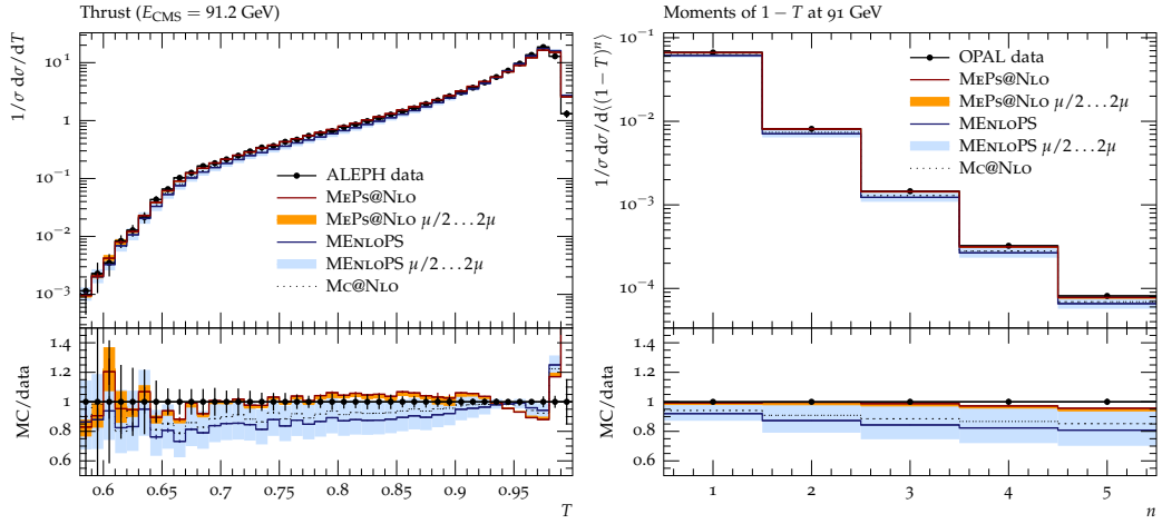
Figure 3: Perturbative uncertainties in MENLOPS and MEPS@NLO predictions of thrust. Compared are the measurements for the event shape from ALEPH [35] and its moments from OPAL [36].
