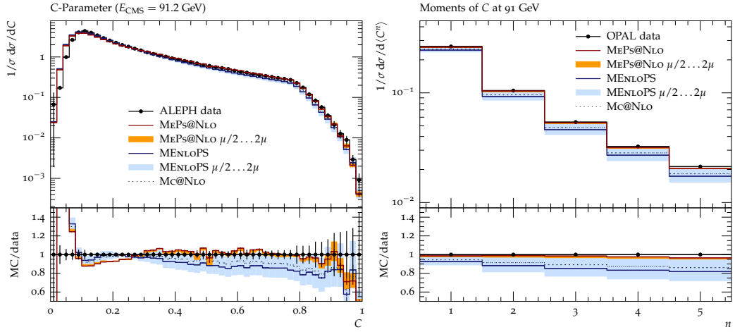
Figure 6: Perturbative uncertainties in MENLOPS and MEPS@NLO predictions of the C -parameter. Compared are the measurements from ALEPH [35] and OPAL [36].
