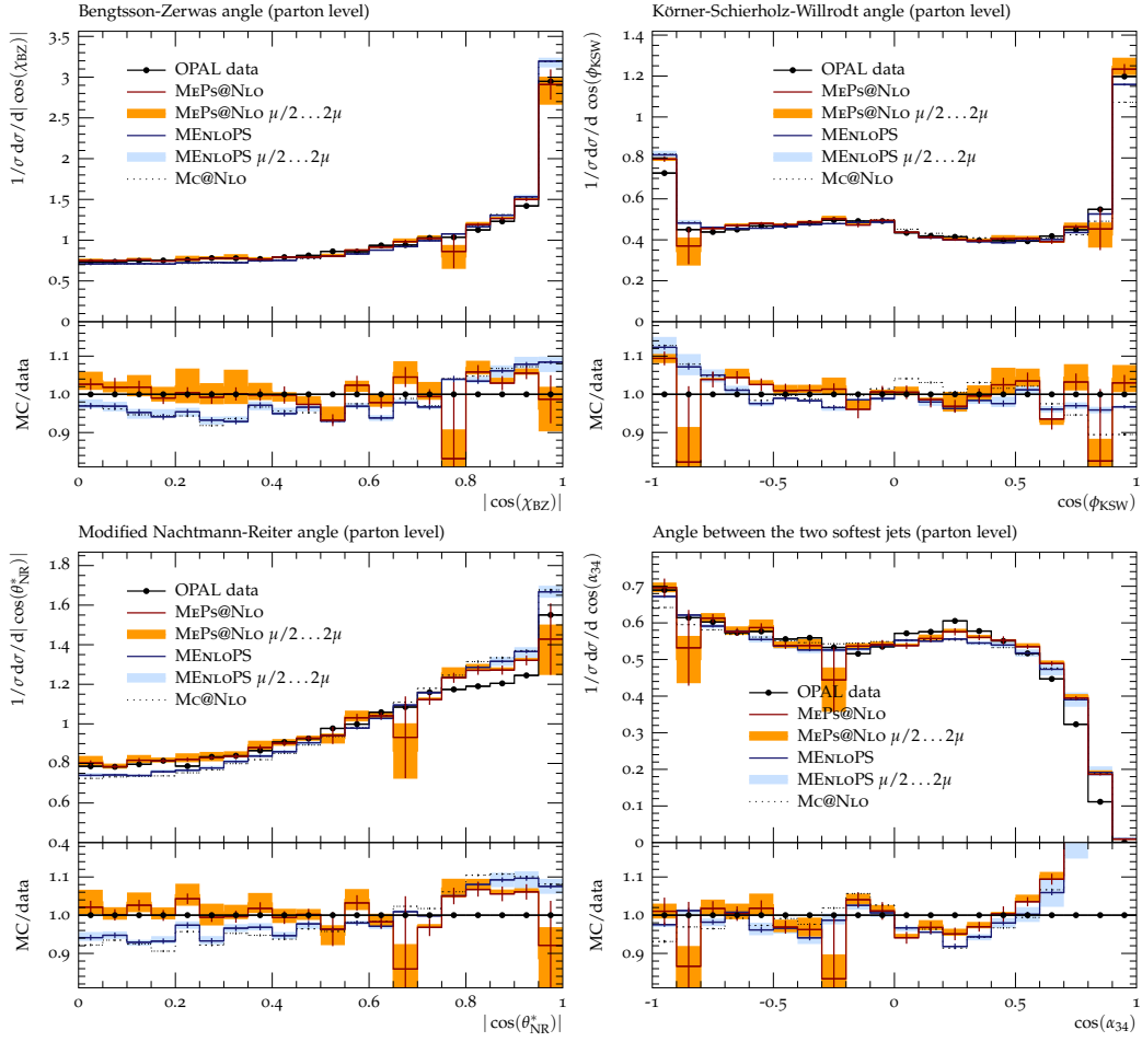
Figure 8: Four-jet angles using the Durham algorithm compared to data from OPAL [37].
