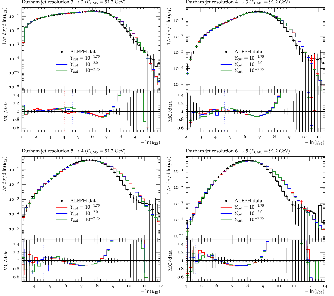
Figure 1: Experimental data from ALEPH [35] for the differential (n+1) \rightarrow n jet rates with n = \{2, 3, 4, 5\} (upper and lower panel, left to right) at the Z pole ( E_{\text{c.m.}} = 91.2 GeV) are compared with MEPS@NLO simulations with different values of the merging cut, Y_{\text{cut}} = 10^{-\{1.75, 2.0, 2.25\}} . To guide the eye, the merging cuts have been indicated with dotted lines in the same colour in the ratio plot.
