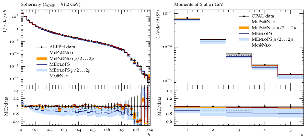
Figure 7: Perturbative uncertainties in MENLOPS and MEPS@NLO predictions of sphericity. Compared are the measurements from ALEPH [35] and OPAL [36].
