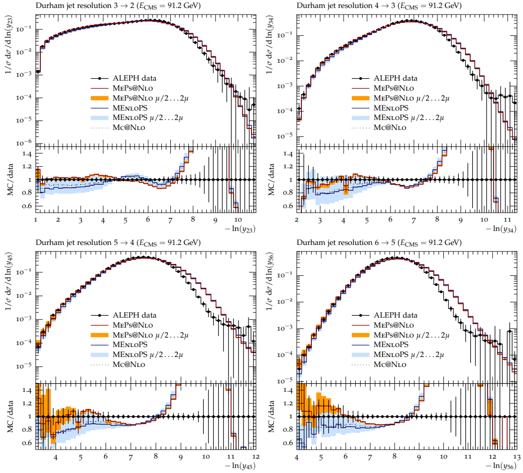
Figure 2: Perturbative uncertainties in MENLOPS and MEPS@NLO predictions of differential jet rates compared to data from ALEPH [35].
