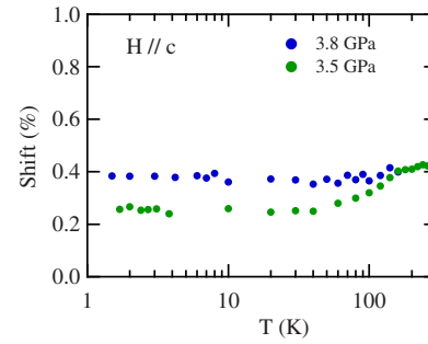
FIG. 3. (Color online) Knight shift of ^{63}\text{Cu} nuclei for the ladder sites at low temperatures derived from high fields.
