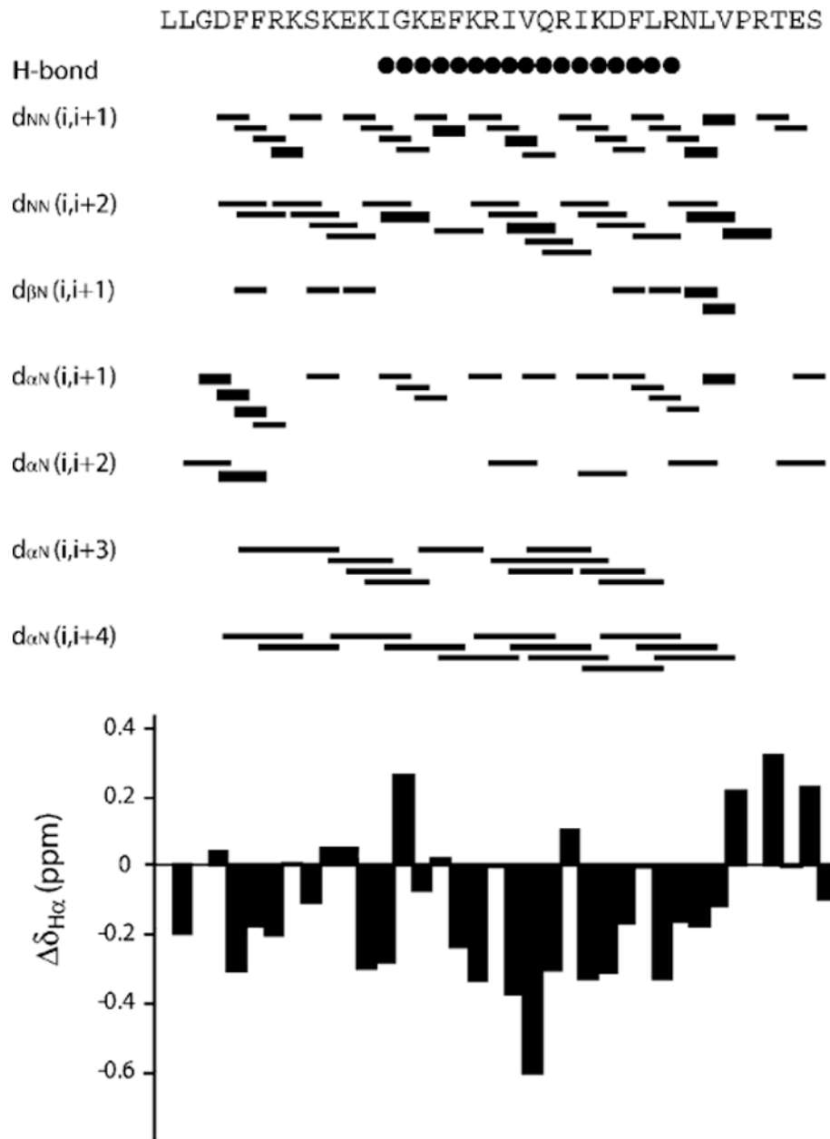
Figure 3. Summary of the backbone NOESY cross-peaks, H_{\alpha} CSI, and H/D exchange experiments.
