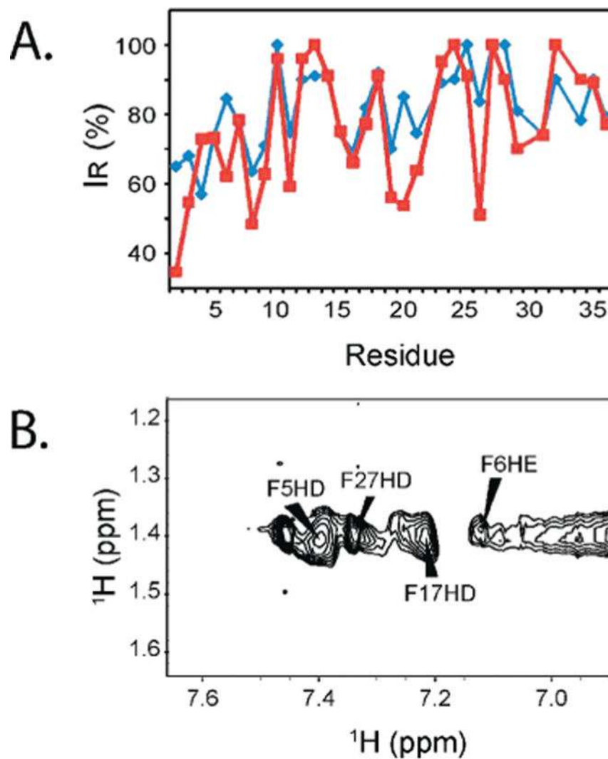
Figure 7. (A) Intensity retention ( I_R ) plots for H_\alpha of LL-37 in the presence of 1:2 (blue trace) and 1:4 (red trace) peptide to Gd^{3+} ratios. (B) Selected region of the NOESY spectrum showing the NOEs between the aromatic residues and the methylene detergent resonances.
