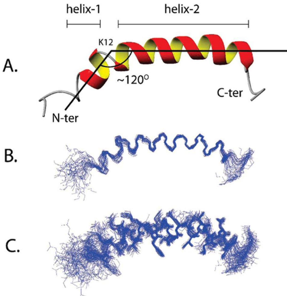
Figure 5. (A) Representative structure of LL-37 showing the angle between the two helical domains and the break point centered at K12. (B) Ensemble of conformers for LL-37 showing the convergence of the conformers for backbone atoms. (C) Heavy atom representation of the final calculated ensemble of conformers showing the convergence of the side chains. The structures were fit onto the relaxed average conformation.
