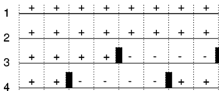
FIG. 12. Refocusing scheme for a four-spin system, designed to leave J_{12} active the whole time but to neutralize the effect of the other J_{ij} . The interval is divided into slices of equal duration, and the “+” and “-” signs indicate whether a spin is still in its original position, or upside down. The black rectangles represent 180^\circ pulses, which flip the corresponding spin.
