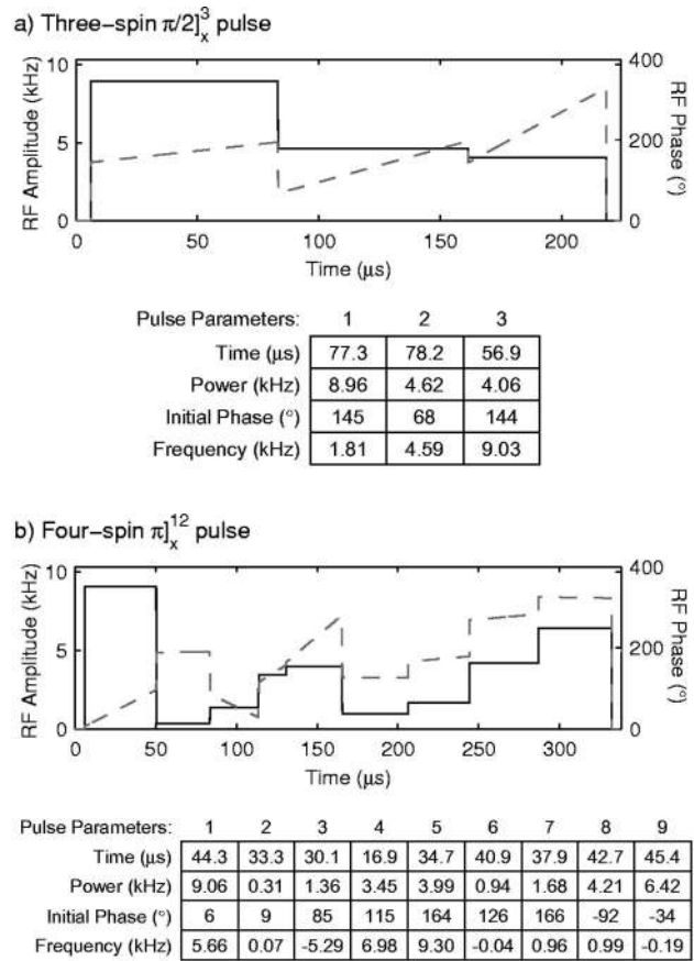
FIG. 27. The ideal RF waveform for two examples of strongly modulated pulses: solid lines, amplitude of the waveform; dashed lines, phase. Details of the pulse parameters, as in Eq. (55) are listed below each wave form. The 6- \mu s time interval with zero RF power before and after the composite pulses is needed due to experimental implementation issues. The composite pulse in (a) performs a 90^\circ rotation on one of the ^{13}\text{C} nuclei of ^{13}\text{C} -labeled Alanine and the pulse in (b) performs a simultaneous 180^\circ rotation on two ^{13}\text{C} nuclei of ^{13}\text{C} -labeled Crotonic acid. Courtesy of D. G. Cory. Reproduced from Fortunato et al. , 2002.
