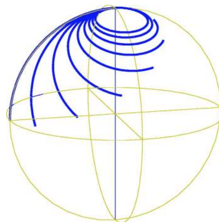
FIG. 8. (Color in online edition) Trajectory in the Bloch sphere described by a qubit initially in |0\rangle (along +\hat{z} ), after a 250- \mu s pulse of strength \omega_1 = 1 kHz is applied off-resonance by 0, 0.5, 1, ..., 4 kHz. On-resonance, the pulse produces a 90° rotation. Far off-resonance, the qubit is hardly rotated away from |0\rangle .
