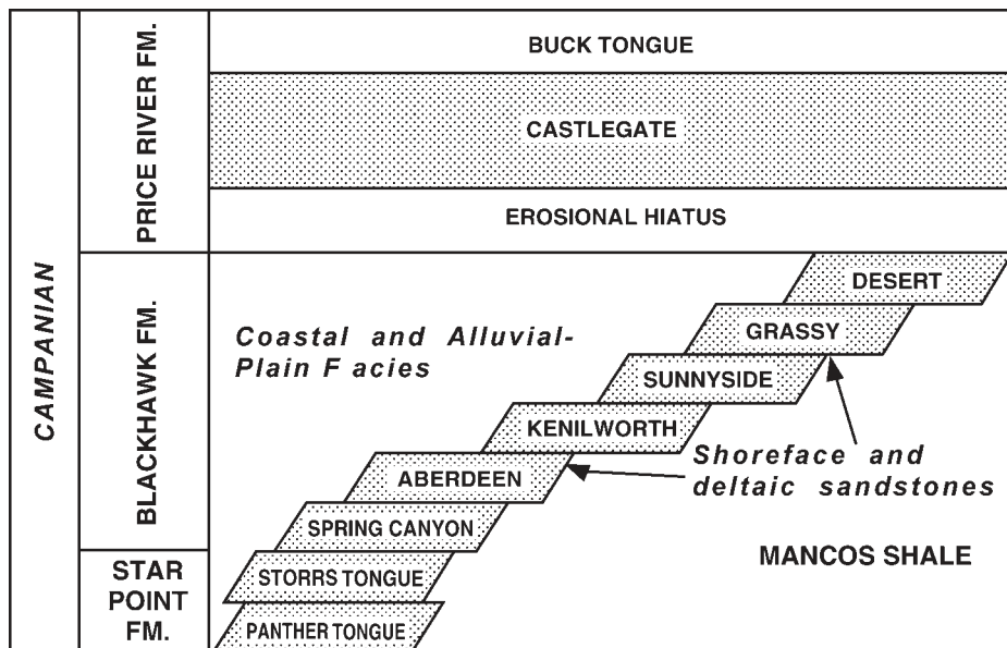
FIG. 2.—Schematic west-to-east Blackhawk–Castlegate stratigraphy (Taylor and Lovell 1995, modified from Young 1955).
