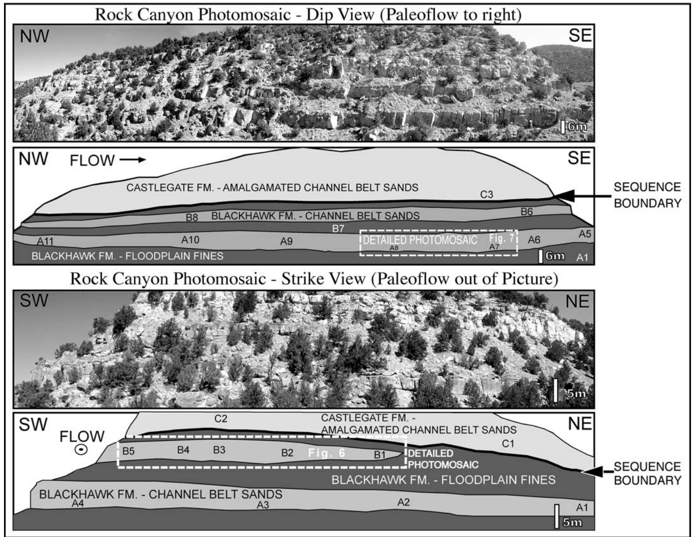
FIG. 5.—Regional depositional dip- and strike-oriented photomosaics with interpretations of channel-belt sandstones and floodplain facies. Amalgamated channel belts at the top of the outcrop represent the Castlegate sandstone. Channel belts in the Blackhawk are single story and average about 5 m thick. Individual segments of the channel belts were selected for detailed analysis of bar and bedding geometry (see Figs. 6, 7). A1, B1 etc. represent locations of measured sections. Locations of photomosaics are shown in Figure 1.
