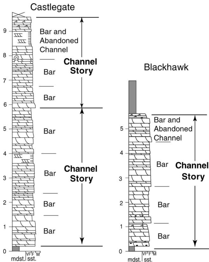
FIG. 11.—Side-by-side comparison of Blackhawk and Castlegate measured sections show extreme similarity in thicknesses of cross-sets, and bar and channel thicknesses. The Castlegate shows a greater degree of amalgamation of channels and channel belts.
