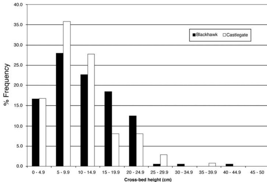
FIG. 8.—Histograms of cross-stratal thicknesses between Blackhawk and Castlegate channels.
