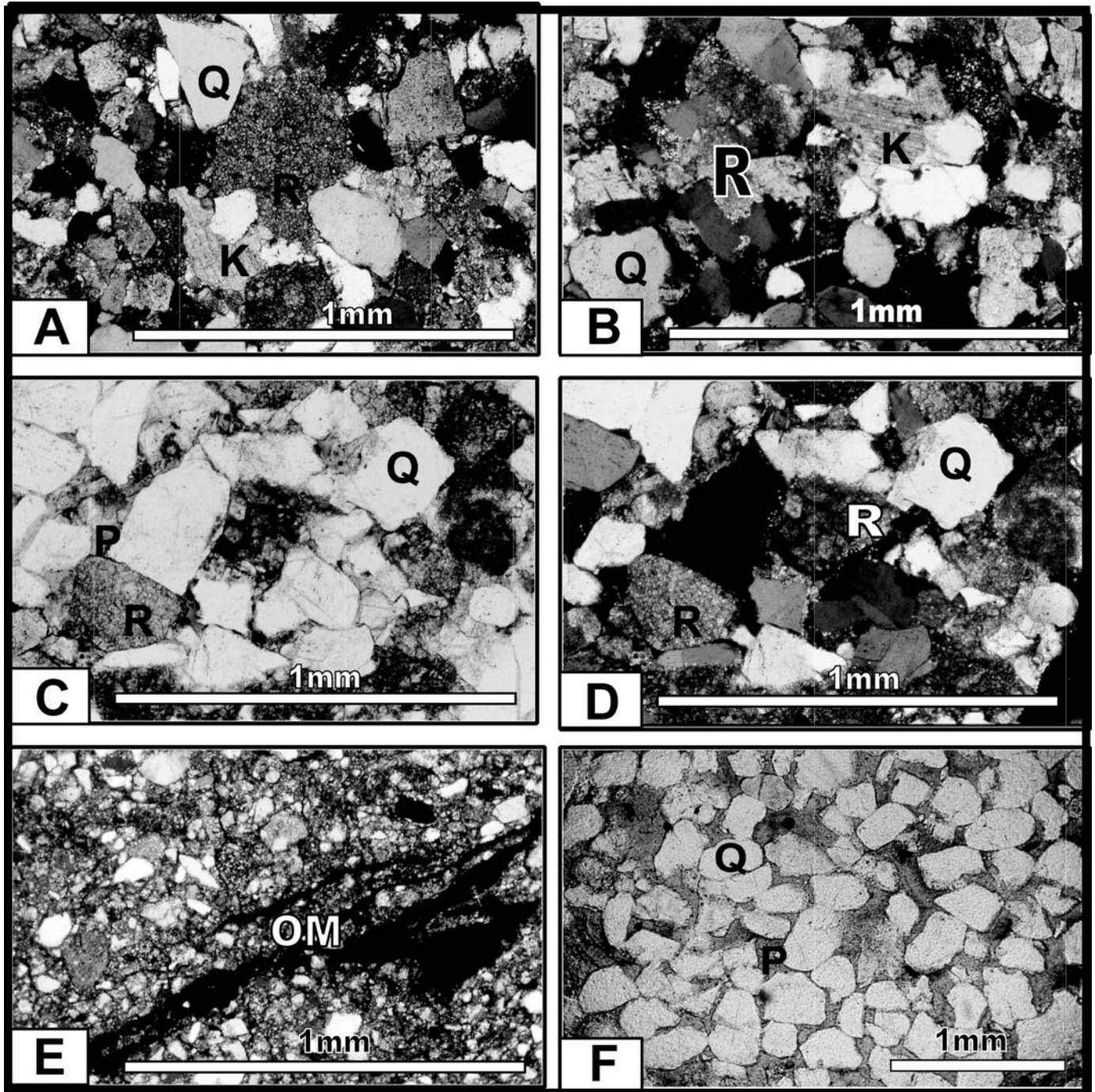
FIG. 10.—Photomicrographs of Blackhawk and Castlegate. Q = Quartz; K = Potassium Feldspar; R = Rock fragment; P = Pore space; OM = Organic matter. Scale bar is 1 mm. A) Blackhawk lith-arenite, showing moderate sorting and abundance of labile grains. Cross-polarized light. B) Blackhawk lithic felds-arenite, showing rock fragments and feldspars in cross-polarized light. C) Blackhawk lithic felds-arenite with carbonate and other sedimentary rock fragments in plane-polarized light. Note carbonate rhomb in the right rock fragments. Same slide as Part D. D) Blackhawk lithic felds-arenite in cross-polarized light. Same slide as in Part C. E) Blackhawk siltstone in crossed polarized light. Note large elongate fragment of dispersed organic matter. F) Castlegate quartz-arenite is composed predominantly of well-rounded quartz grains (plane-polarized light). Note high porosity and lack of labile grains. Quartz is assumed to be derived from the uplifted Permian–Pennsylvanian Oquirrh eolianites (Horton et al. 2004).
