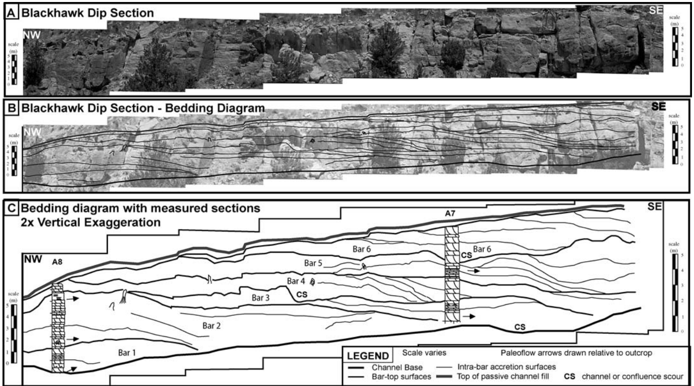
FIG. 7.—Dip-oriented bedding diagram showing interpretation of bars and channels. Downstream dipping surfaces indicate downstream accreting bars. CS refers to interpreted channel or confluence scours. Measured sections in lowest panel show vertical facies successions. Measured sections are in meters. Arrows represent paleocurrents. Down is towards viewer, up is away from viewer, and left and right represent flow to the left or right, respectively. Legend for measured sections is provided in Figure 9. Location of photomosaic is shown in Figure 5. See text for further explanation.
