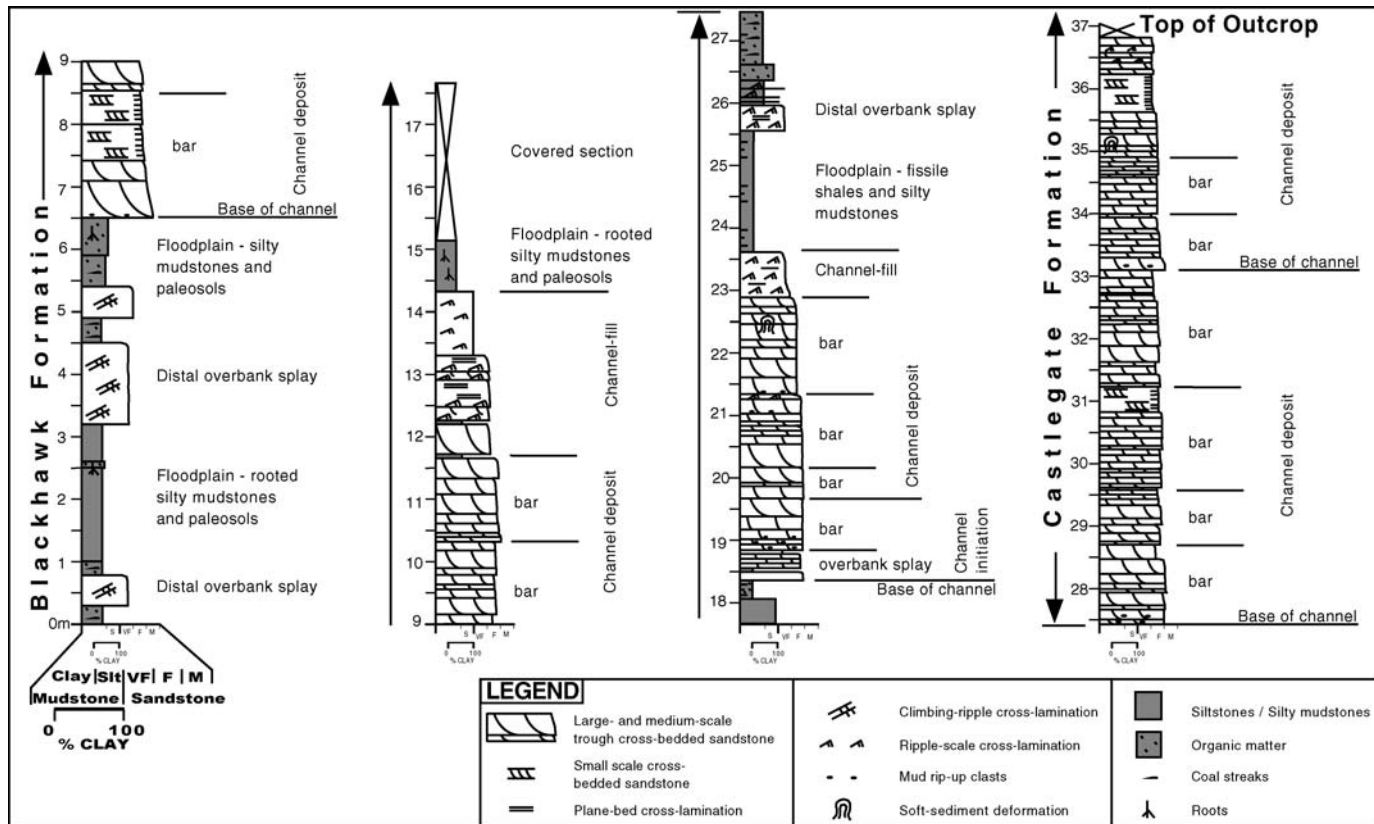
FIG. 9.—Measured section of entire outcrop, showing alternation of channel and floodplain facies. Upper 9 meters represents lower Castlegate Formation.
