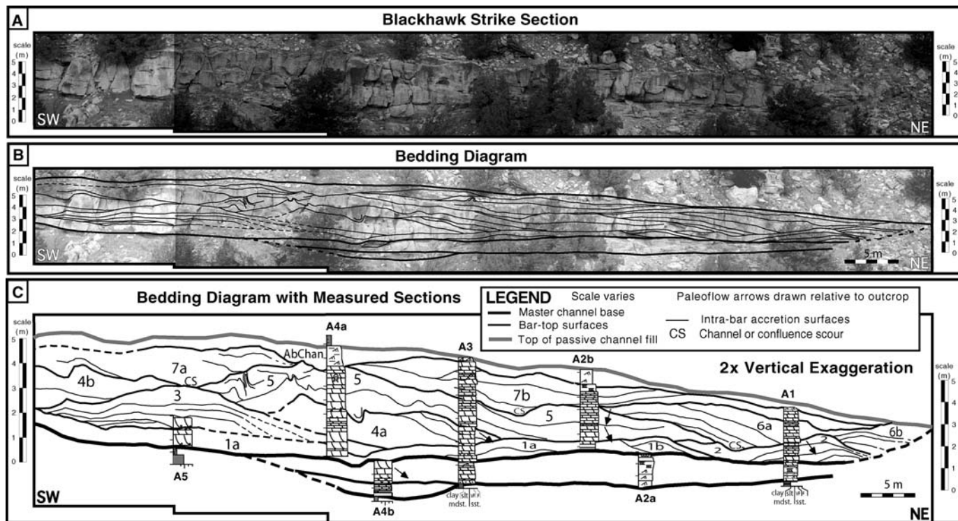
FIG. 6.—Strike-oriented bedding diagram showing interpretation of bars and channels. Mounded geometries clearly indicate braid bars. Bars are numbered 1 to 7. Measured sections in the lowest panel show vertical facies successions. Measured sections are in meters. Arrows represent paleocurrents. Down is towards viewer, up is away from viewer, and left and right represent flow to the left or right, respectively. Legend for measured sections is provided in Figure 9. Location of photomosaic is shown in Figure 5. See text for further explanation.
