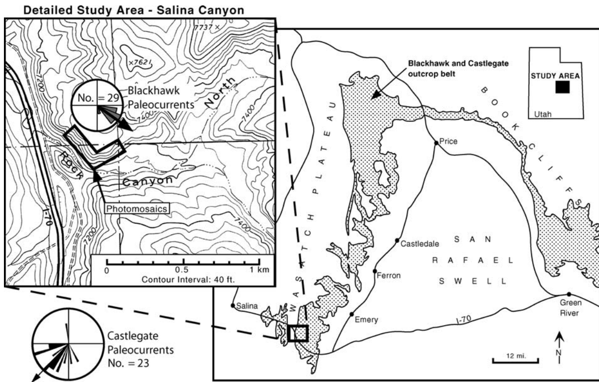
FIG. 1.—Location of the Study Area. Stippled area shows the location of the Blackhawk and Castlegate outcrop belt. Inset shows topographic map of Rock Canyon area. Rose diagrams show paleocurrent data from the Castlegate and the Blackhawk formations in the study area.
