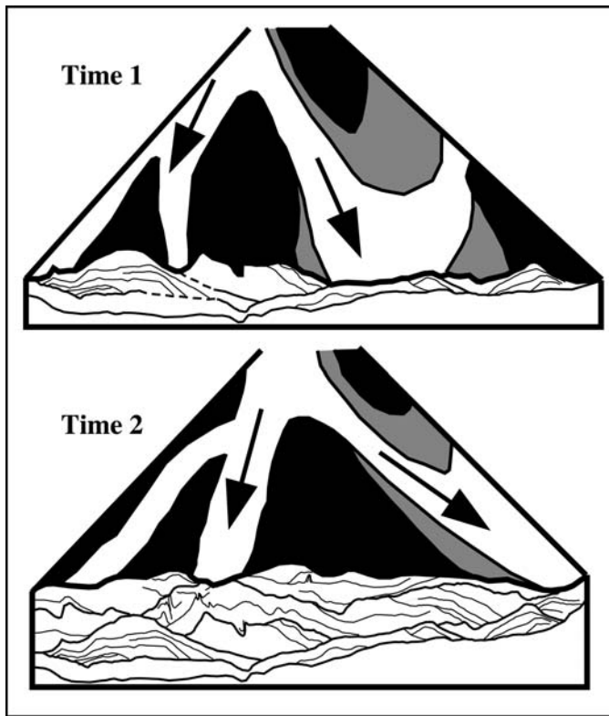
FIG. 12.— Reconstruction of Blackhawk braid bars based on strike bedding diagram (Fig. 6). Time 1 depicts deposition associated with bars 1–4a, and time 2 depicts deposition associated with bars 7a and 7b. Note overlapping and alternating bar stacking pattern. Black represents subaerial bar, light gray represents subaqueous bar.
