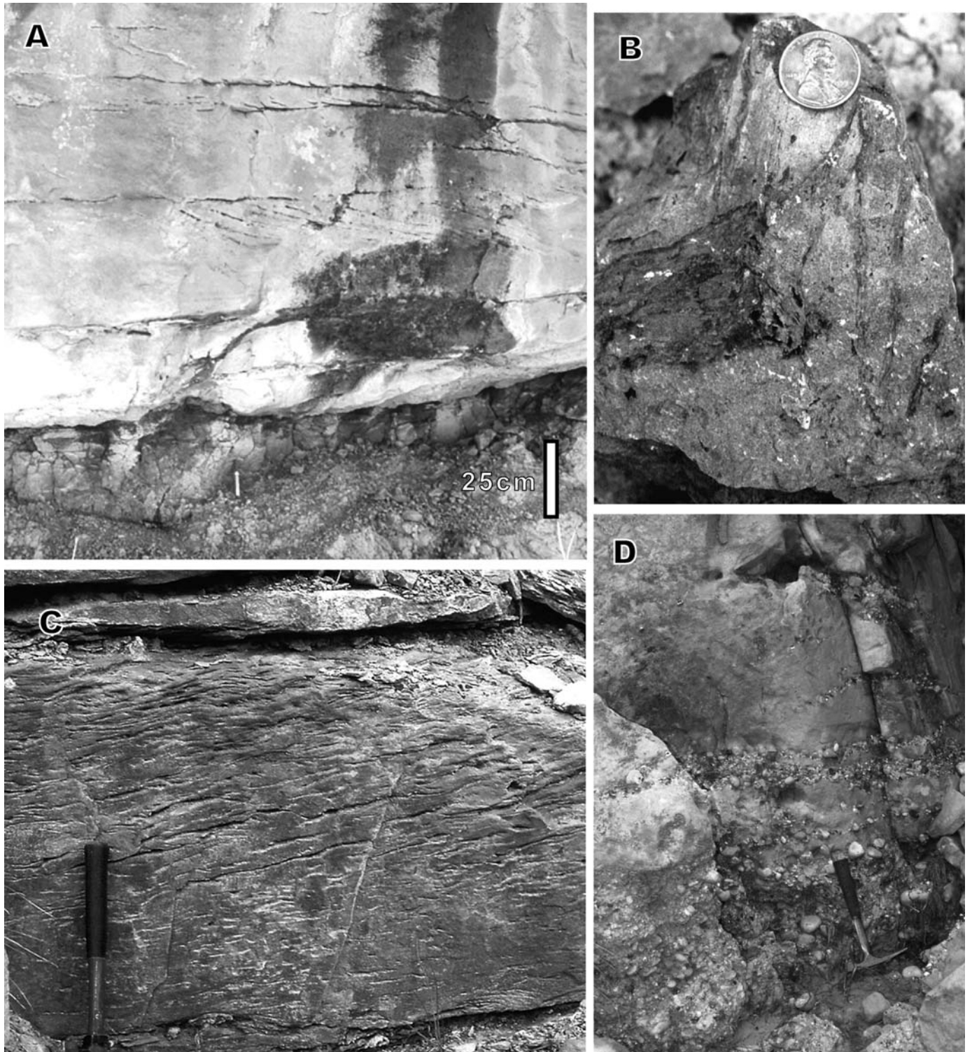
FIG. 4.—Photographs of facies, A ) base of a Blackhawk channel showing dune-scale cross-bedded sandstones eroding into underlying gray floodplain mudstones. B ) Close-up of mudstones showing root traces and preserved organic plant material. Penny for scale. C ) Climbing-ripple sandstones within Blackhawk floodplain, interpreted as crevasse-splay deposits. Note hammer for scale. D ) Pebble conglomerate grading into dune-scale cross-bedded sandstones within the Castlegate. Note hammer for scale.
