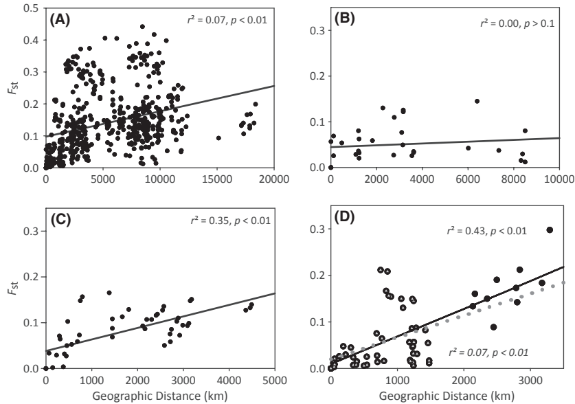
Fig. 4 Isolation-by-distance patterns in Porites lobata . Geographical distance explained 7% of the variation in genetic distance ( F_{st} ) across all sampling site, none of the variation in the western central Pacific (b), and 35% of the variation in the eastern central Pacific (c). Geographical distance explained 43% of the variation in genetic distance among all sites in the Eastern Tropical Pacific (d) black circles and regression line) and 7% of the variation when excluding Clipperton (d, grey triangles and dotted regression line). Note differences in axis scales among panels.
