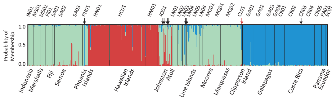
Fig. 7 When treated as genotypes of unknown origin, four Clipperton genotypes (red arrow) assigned with high probability (mean CP = 0.84 \pm 0.09 ) to the central Pacific ( K = 3 ) and one genotype appeared admixed between CP (assignment probability = 0.36) and EP (0.62). Structure identified seven genotypes from the central Pacific (one from PH01, four from JO01, two from LN04) and one genotype from the eastern Pacific (CR03) as first generation migrants (black arrows) with high probability ( >0.9, P < 0.001 ). Model assumed admixed populations, correlated allele frequencies and K = 3 .
