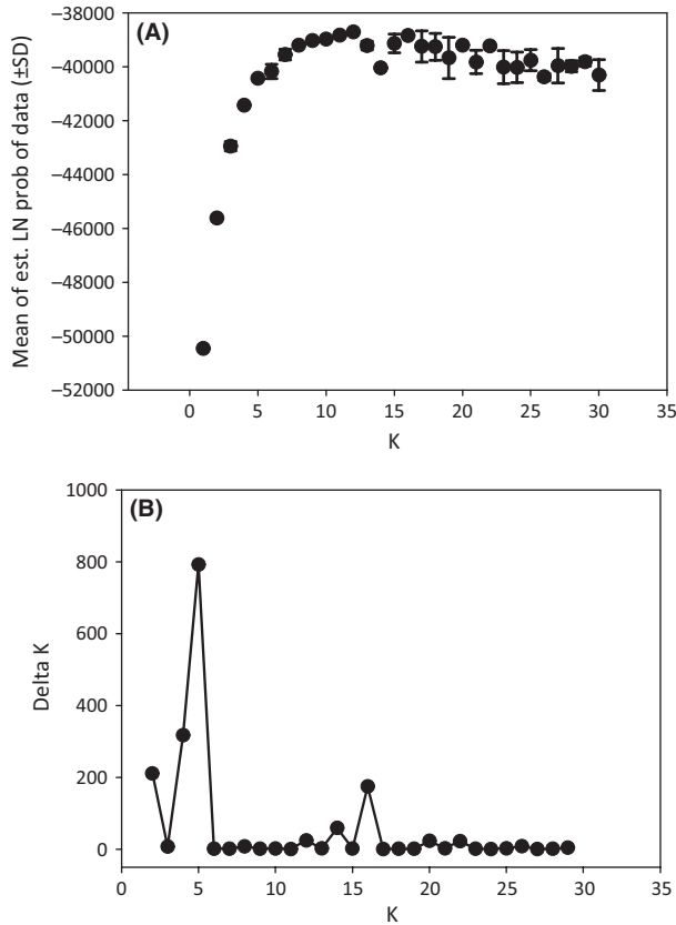
Fig. 6 Mean log-likelihood of K (a) and Delta K (b) values for STRUCTURE analysis of Porites lobata samples, pacific-wide.
