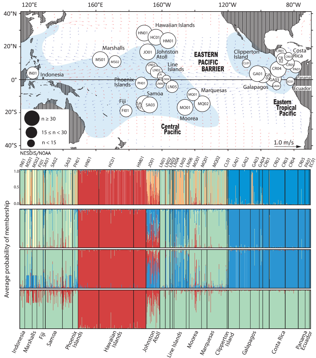
Fig. 1 Porites lobata population structure across the central and Eastern Tropical Pacific. The size of the circles is proportional to the sample size ( n , chart inset) collected at each location. Bar graphs show the average probability of membership ( y -axis) of individuals ( n = 1173 , x -axis) in K = 5 to K = 2 clusters (shown in descending order) as identified by STRUCTURE.
