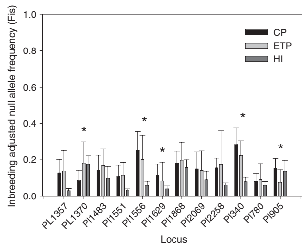
Fig. 2 Porites lobata : Frequency of inbreeding-adjusted null alleles (+1 SD) over 12 loci across the central Pacific (CP), the Hawaiian Archipelago (HI) and the Eastern Tropical Pacific (ETP). A Kruskal–Wallis one-way analysis of variance indicated differences in null allele frequency within loci across regions (asterisk, P < 0.05 ).
