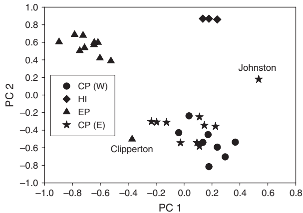
Fig. 5 Principal component analysis of allele frequency covariance in Porites lobata populations. 31 of 229 Principal component analysis (PCA)-axes were retained, explaining 100% of the cumulative variance. Plotted are the first two axes explaining 47.73% ( P < 0.05 ) and 28.9% ( P < 0.05 ) of the variance, respectively. central Pacific West [CP (W), circles], central Pacific East [CP (E), stars], Hawaii (HI, diamonds), eastern Pacific (EP, triangles).
