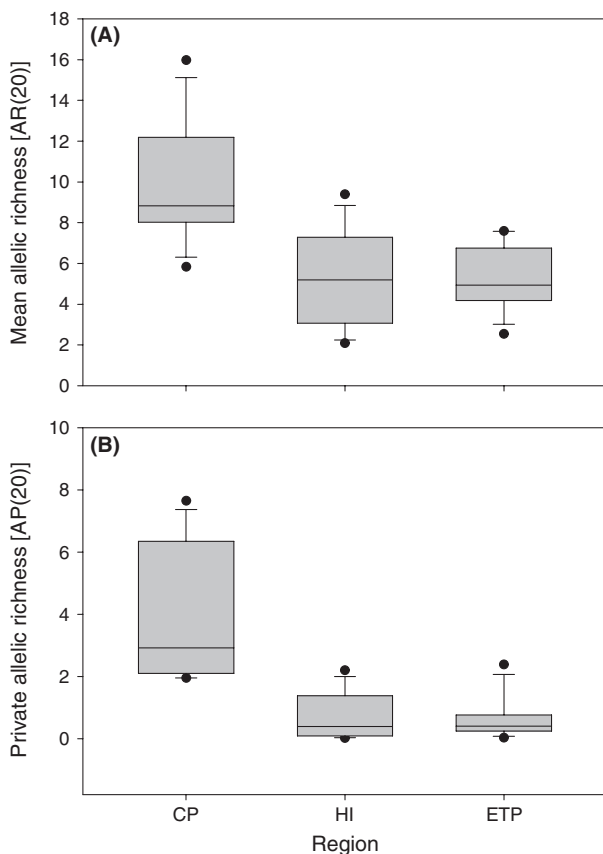
Fig. 3 Porites lobata mean allelic richness (AR(20)) and private allele richness (AP(20)) rarefied to a sample size of three sites per region and 20 genes per site. A Kruskal–Wallis one-way analysis of variance indicated differences across regions ( P < 0.01 ) for both AR(20) and AP(20). CP = central Pacific, HI = Hawaiian Islands, ETP = Eastern Tropical Pacific.
