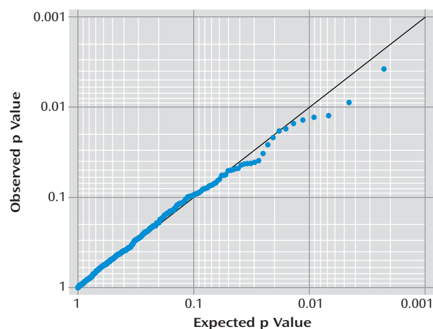
FIGURE 2. Quantile-Quantile Plot of Observed Versus Expected p Values for Tag Single Nucleotide Polymorphisms (SNPs) a
