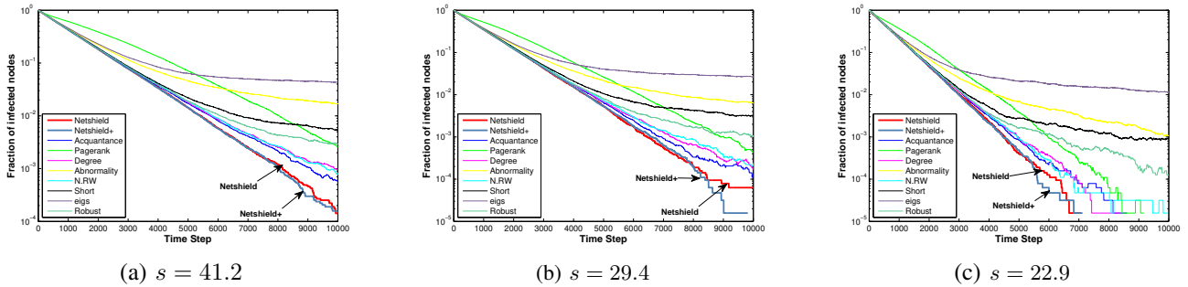
Fig. 4: Evaluation of immunization of NetShield and NetShield+ on the Oregon-A graph. The fraction of infected nodes (in log-scale) vs. the time step. s is normalized virus strength. Lower is better. The proposed NetShield and NetShield+ is always the best, leading to the fastest healing of the graph. Best viewed in color.
