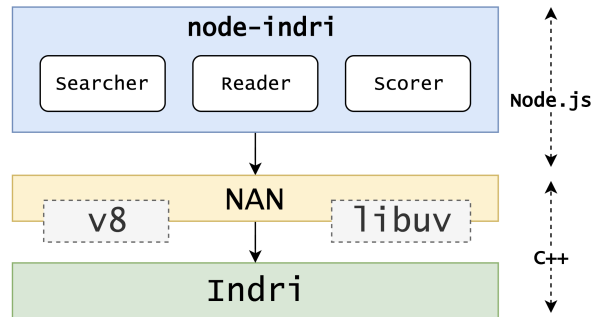
Fig. 1. Overview of node-indri layers of abstractions and their implementation languages and platforms.
