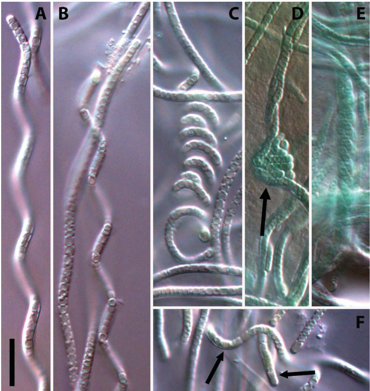
FIGURE 2. Main characteristics of Nodosilinea chupicuarensis . A-C. Mature filaments forming loose to tight spirals. D. A characteristic nodule (arrow). E. Multiserial filament. F. Filaments with mature, elongated end cells (arrows). All figures to same scale, scale = 10 \mu m.
