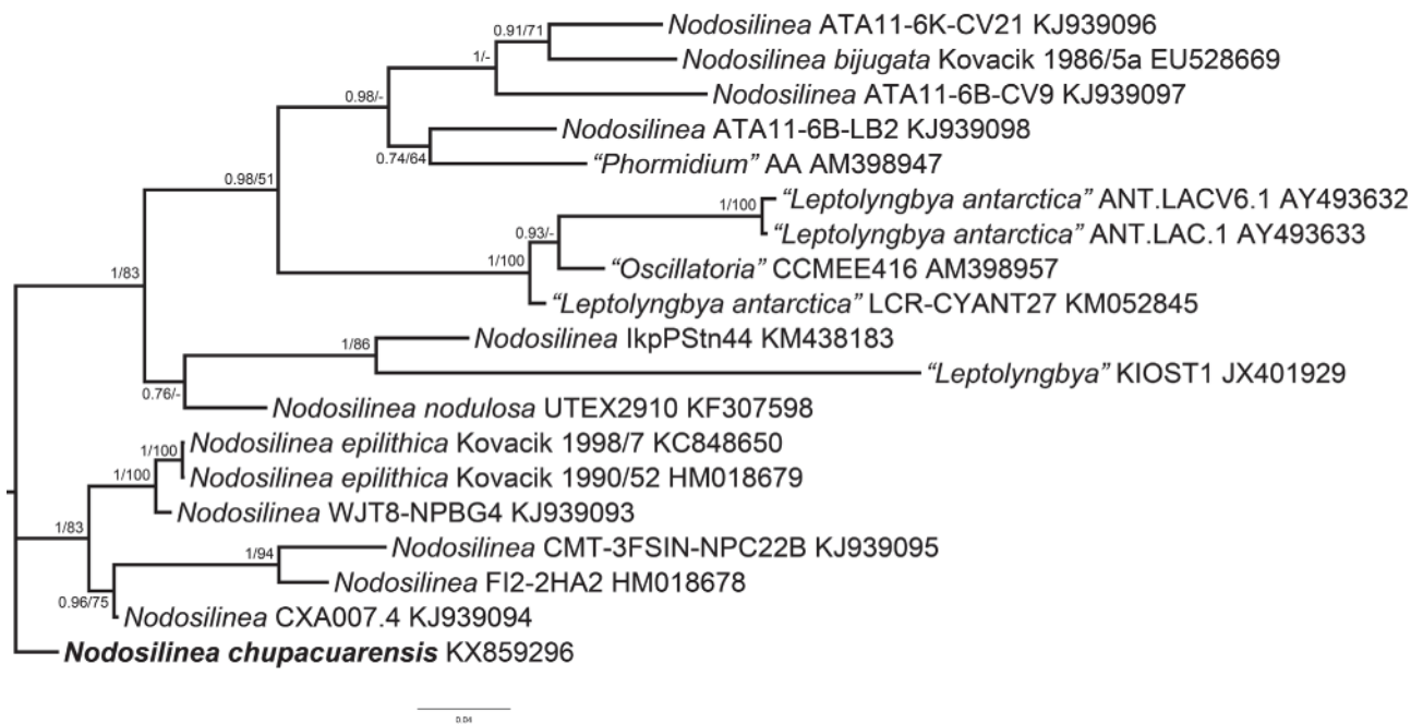
FIGURE 5. Unrooted tree of Nodosilinea strains based on Bayesian Analysis of 19 sequences (562 DNA positions, 114 coded indels). Bootstrap values from the parsimony analysis (562 DNA positions, gaps coded as a fifth base) are mapped onto the nodes in which the analyses were in agreement.
