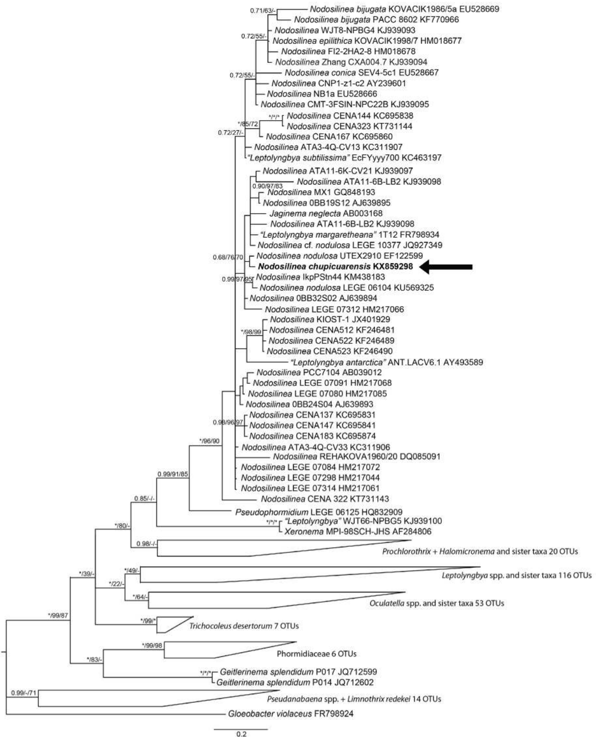
FIGURE 4. Phylogenetic position of Nodosilinea chupicuarensis (denoted with an arrow) in a Bayesian Analysis (285 OTUs, 1222 positions), with support values on nodes representing BA posterior support/ML bootstrap support/MP bootstrap support, respectively. The uncollapsed tree from which this figure was derived appears in supplemental materials.
