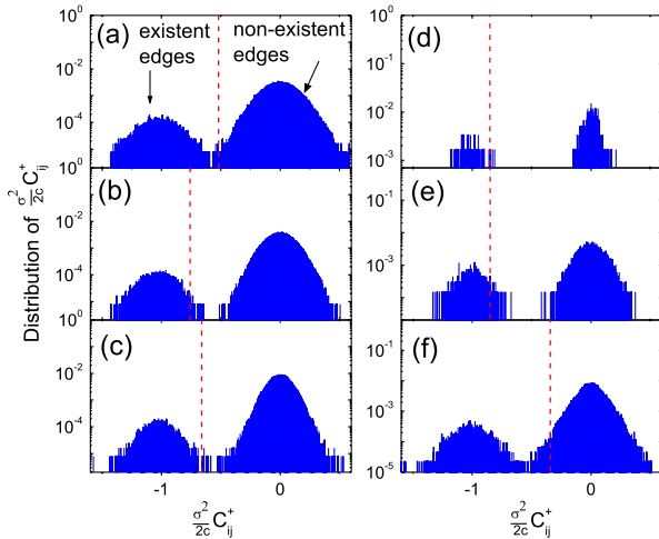
FIG. 1 (color online). Distribution of the values of [\sigma^2/(2c)]C_{ij}^{\dagger} , where C_{ij}^{\dagger} are the elements in the pseudo inverse matrix of the dynamical correlation matrix \hat{C} . Consensus dynamics [15] are used for (a) random [21], (b) small-world [22], (c) scale-free model networks [23] and three real-world networks: (d) friendship network of karate club [25], (e) network of American football games among colleges [26], and (f) the neural network of C. Elegans [22]. The theoretical threshold [\sigma^2/(2c)]C_M^{\dagger} is marked by red dashed lines. The sizes of model networks are all 500. For random networks, the connection probability among nodes is 0.024. For scale-free networks the minimum degree is k_{\min} = 6 . For small-world networks, \langle k \rangle = 12 and the rewiring probability is 0.1.
