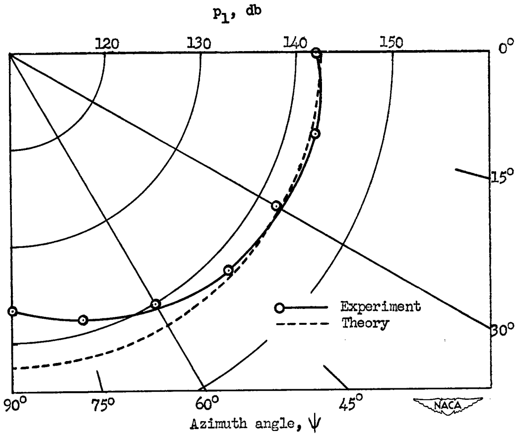
Figure 6.- Angular distribution of pulsejet fundamental. 100 percent rated thrust (90 lb); \frac{Z}{D} = 20 .
