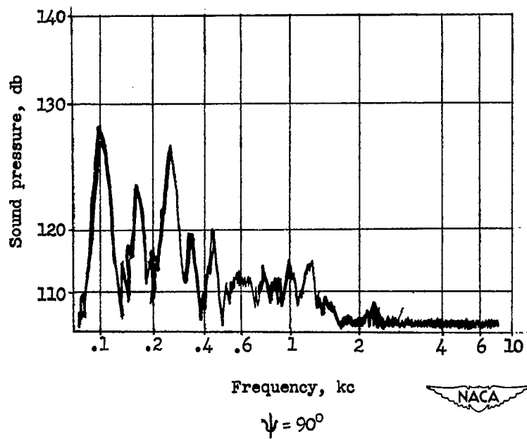
Figure 8.- Ramjet noise spectrums. 80 percent rated thrust (22.4 lb);
