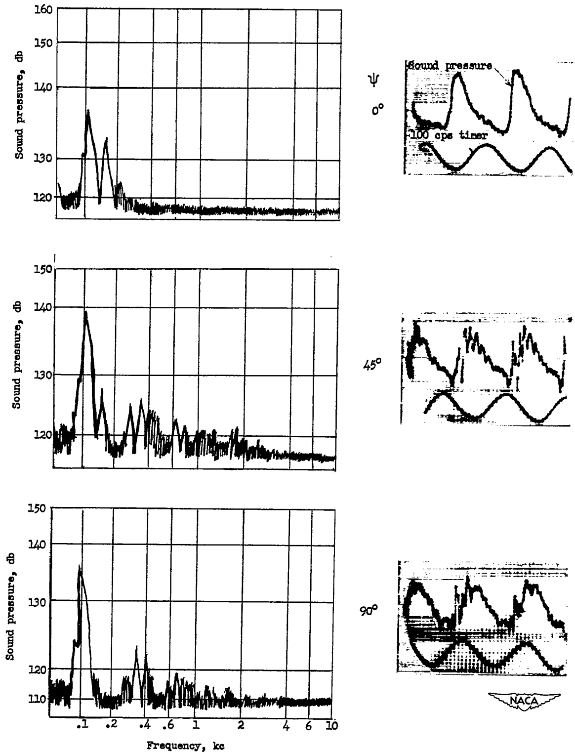
Figure 5.- Pulsejet noise spectrums and wave forms. 80 percent rated thrust (72 lb); \frac{Z}{D} = 20 .
