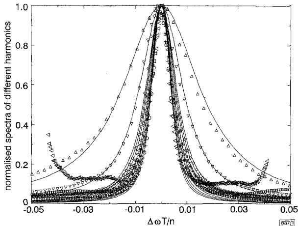
Fig. 1 Normalised intensity spectra of different harmonics against offset frequency divided by harmonic number n
