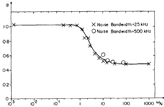
Fig. 9. Measured values of parameter \alpha versus normalized noise bandwidth \omega_N .
