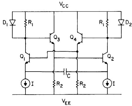
Fig. 1. Cross-coupled relaxation oscillator with floating timing capacitor.
