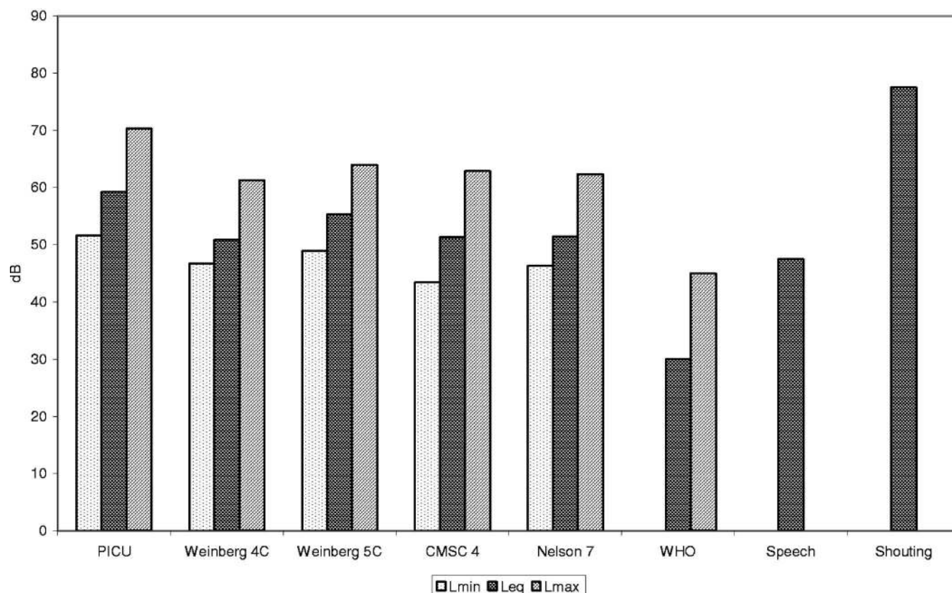
FIG. 9. Logarithmic average A-weighted sound pressure levels measured in JHH compared with WHO guidelines and typical levels for speech.
