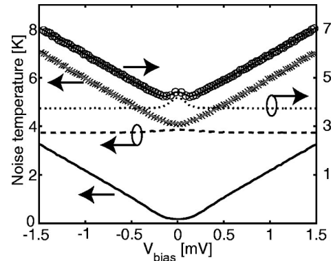
FIG. 11. Measured noise power NP/(k_B BG) in Kelvins at minimum ( \times ) and maximum ( \circ ) Coulomb blockade. The two topmost solid lines correspond to the fits obtained from Eq. (19) using the parameters of Table II. The dashed and dotted lines are amplifier contributions to the measured noise for maximum and minimum Coulomb blockade, respectively. The lowest solid curve illustrates the shot noise contribution to the measured noise.
