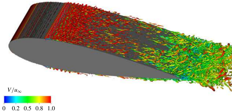
FIGURE 12. (Colour online) Iso-surface of \lambda_2 criterion colour contoured with velocity magnitude for the straight trailing edge.
