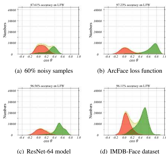
Figure 6. The final \cos\theta distributions of four models (corresponding to four models Figure 2) using our paradigm.
