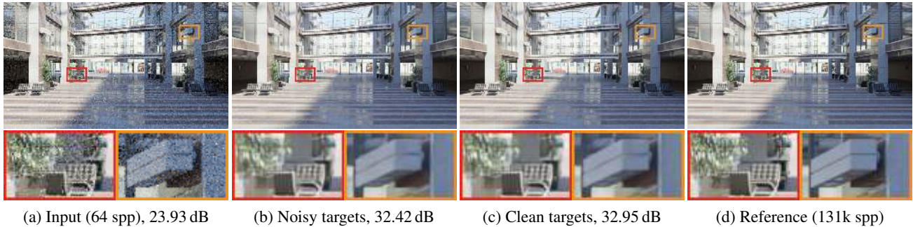
Figure 7. Denoising a Monte Carlo rendered image. (a) Image rendered with 64 samples per pixel. (b) Denoised 64 spp input, trained using 64 spp targets. (c) Same as previous, but trained on clean targets. (d) Reference image rendered with 131 072 samples per pixel. PSNR values refer to the images shown here, see text for averages over the entire validation set.
