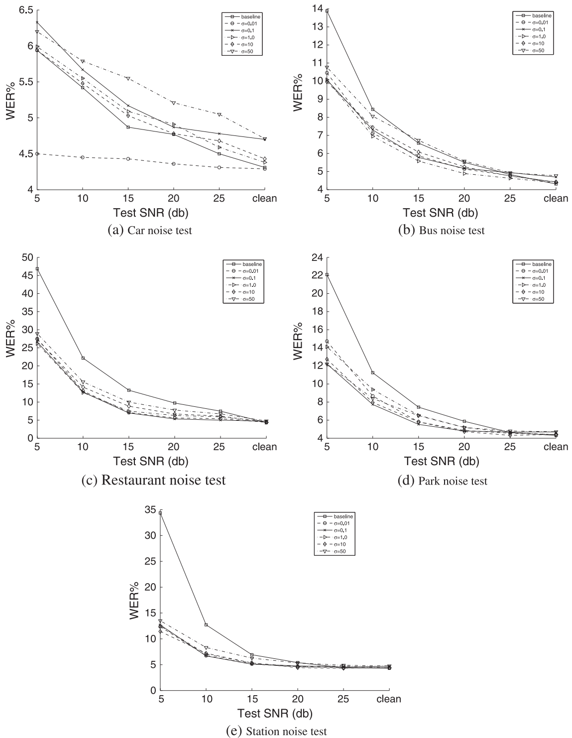
Figure 8 Performance of noise training with different \sigma_{SNR} . (a) Car noise test. (b) Bus noise test. (c) Restaurant noise test. (d) Park noise test. (e) Station noise test. White and cafeteria noises are injected, and \mu_{SNR} = 15 dB. For each plot, the test data are corrupted by a particular 'unknown' noise. The 'baseline' curves present the results of the system trained with clean speech data, as have been presented in Table 1.
