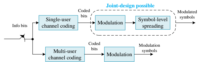
Figure 4 Single-user channel code vs. multi-user channel code based uplink NOMA transmitter for massive IoT
