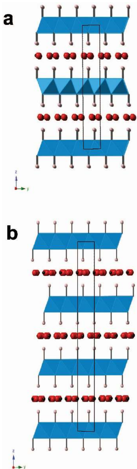
FIG. 2. Hydrotalcite structure viewed down the x axis for (a) 2H_1 polytype with c \sim 16 Å and (b) 3R_1 polytype with c \sim 24 Å. Disordered interlayer carbonate and water is indicated by sheets of carbonate groups (red spheres = oxygen, black = carbon). Note that offset of H atoms across the interlayer is different from that in brucite and that alternate brucite layers are rotated relative to one another about z by 180^\circ in (a), but are translationally equivalent in (b).
