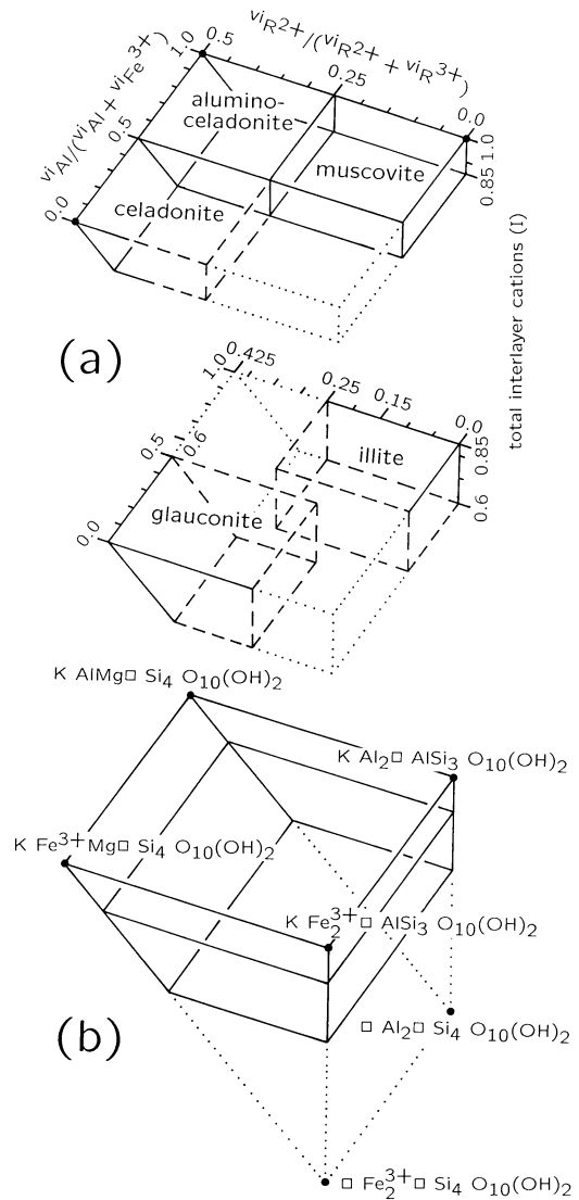
FIG. 1. A three-dimensional plot illustrating the relation of some true dioctahedral micas to interlayer-deficient dioctahedral micas. a. Two slabs cut from the chemographic volume (b) shown in terms of formulas (small solid circles). Dashed lines indicate approximate borders, dotted lines complete the solid. The ratio ^{VI}R^{2+} / (^{VI}R^{2+} + ^{VI}R^{3+}) is equal to x/2 (Table 3) for micas with 2.0 octahedral cations. End-member formulas in (a) are shown by solid circles. Glauconite with \text{Na} > \text{K} should be referred to as “natroglaucosite”.
